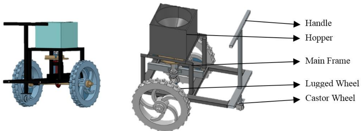
Figure.1. Design of spreader with lugged wheels
