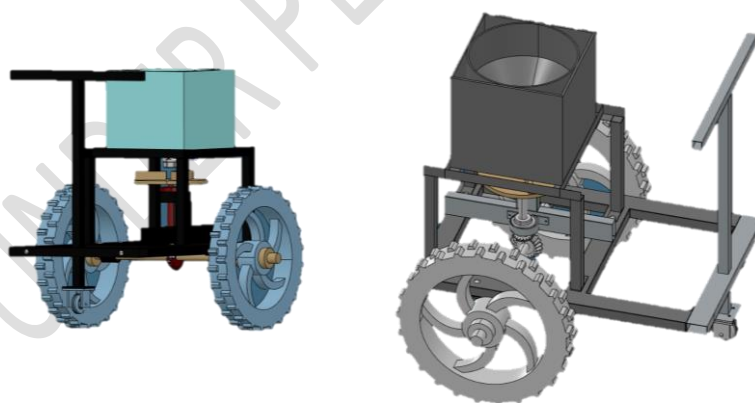
Figure.1. Design of spreader with lugged wheels
