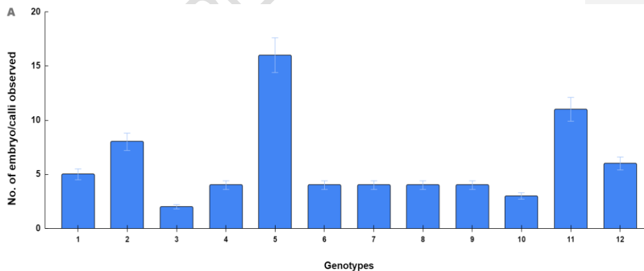
Fig. 3. Effect of plant growth regulators on calli/embryo induction. (A) Analysis of androgenic response among twelve genotypes. [Error bars show mean \pm 1 SE]. (B) Effect of treatments on calli/embryo induction. 1- YP without plant growth regulator; 2-YP+2 mg/l IAA +1 mg/l Kinetin; 3- YP +2 mg/l 2,4D +1 mg/l BAP. [Error bars show mean \pm 1 SD]. Means in the bar graph were separated using Duncan Multiple Range Test at 1% significance. The same variable indicates that the values do not differ significantly.
