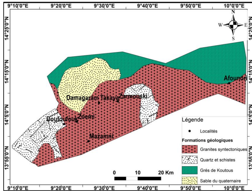
Figure 2: Geology of the study area
