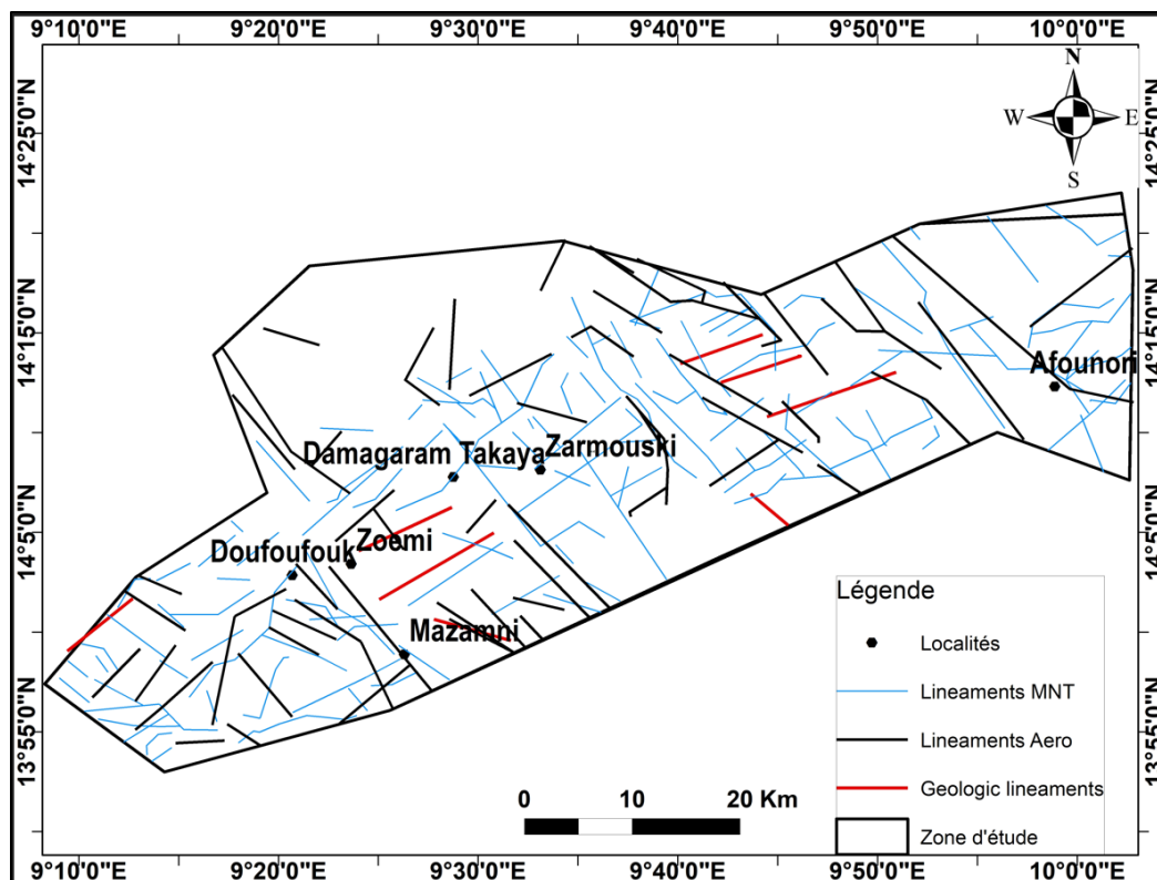
Figure 9: Superposition of lineaments with regional tectonic structures
