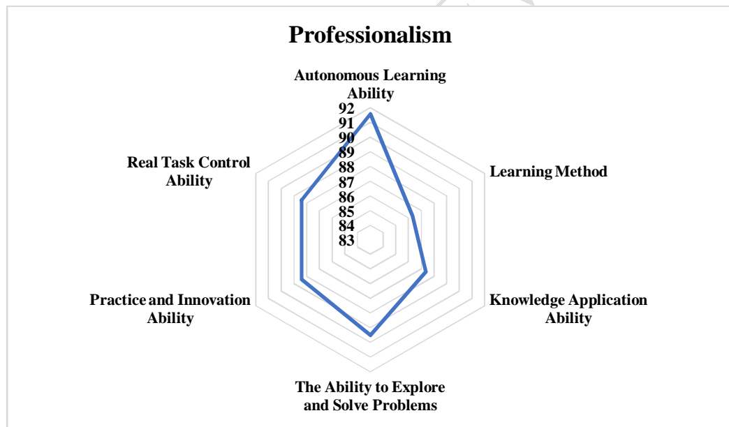
Figure 3: Practice effect investigation
