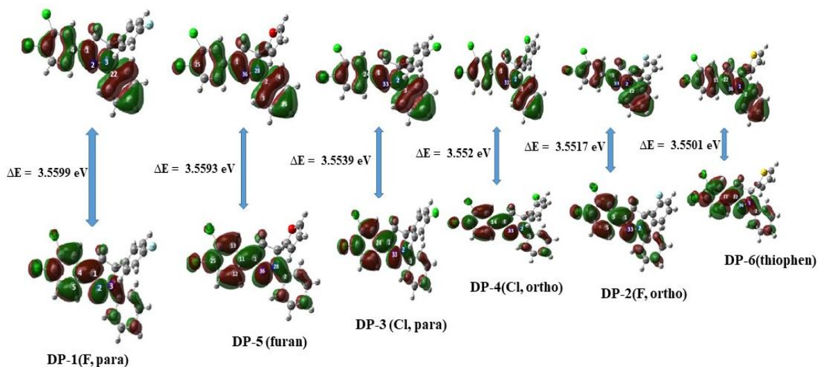
Figure 1: Decreasing order of stability of halogen-substituted dihydropyrazoles according to the energy gap.
