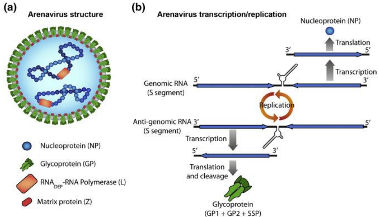
Fig 6: Arenavirus Transcription
