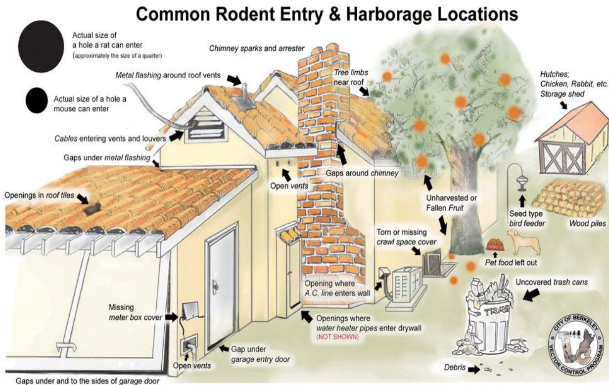
Fig 3: Rodent entry
