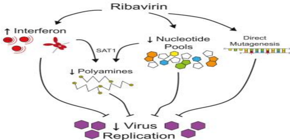
Fig 4: Ribavirin Metabolism
