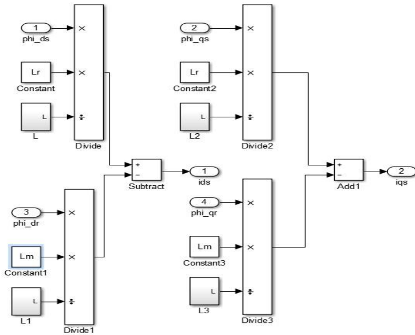
Fig. 6. Subsystem that implements (29) and (30) in Simulink.
