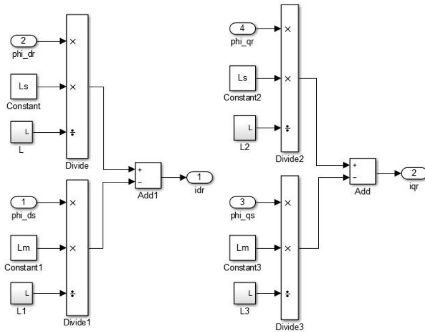
Fig. 7. Subsystem that implements (31) and (32) in Simulink.
