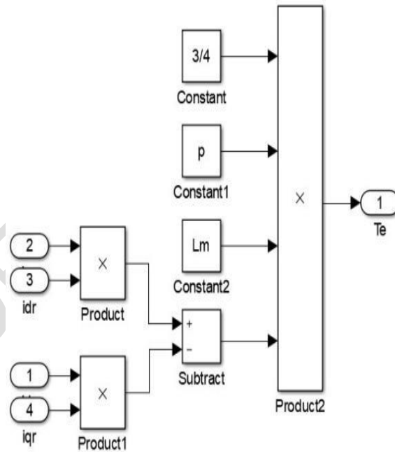
Fig. 9. Subsystem that implements (34).
