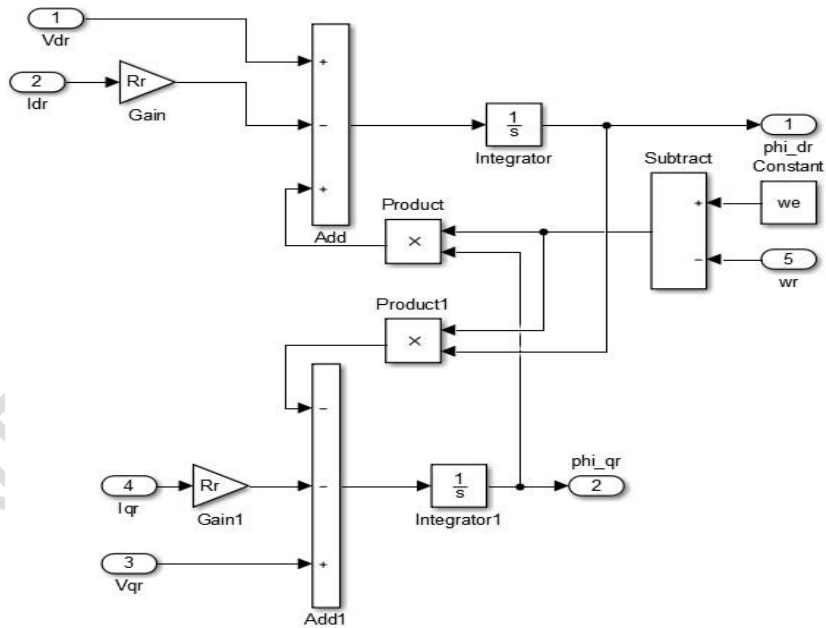
Fig. 5. Subsystem that implements (27) and (28) in Simulink.
