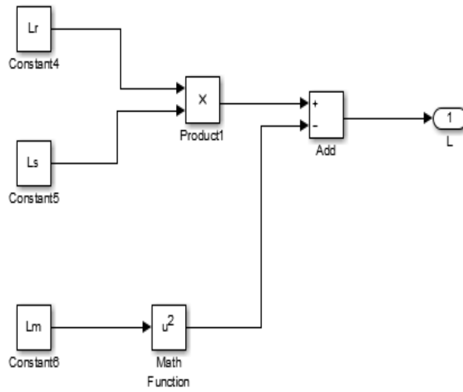
Fig. 8. Subsystem that implements (34) in Simulink.
