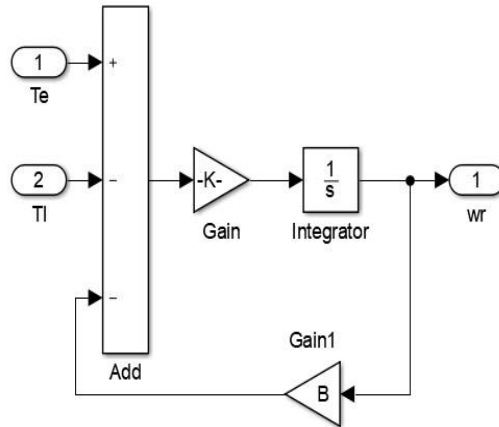
Fig. 10. Subsystem that implements (35) and (36) in Simulink.
