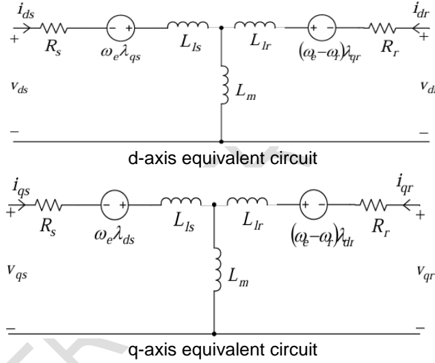
Fig. 2. d-q equivalent circuit of the induction motor [31].
