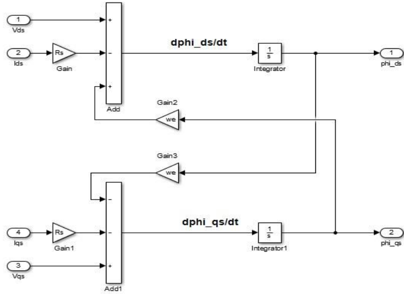
Fig. 4. Subsystem that implements (25) and (26) in Simulink.
