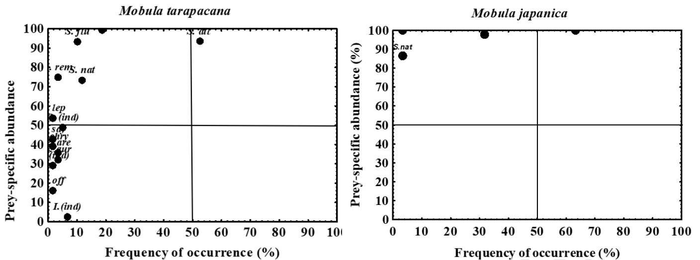
Figure 2. Costello Diagram modified by Amundsen et al. [24] described feeding strategy and niche width of Mobulatarapacana and Mobulajaponica from EEZ Côte d'Ivoire. The points represent different prey types in the stomach contents. Sergestes atlanticus ( S. atl ), Pseudeuphausialatifrons ( P. lat ), Portunussayi ( P. say ), Sargassum natans ( S. nat ), Sargassum fluitans ( S. flu ), Priacanthusarenatus ( P. are ), Remora remora ( R. rem ), Sardinelaureta ( S. aur ), Chloroscombrus chrysurus ( C. chr ), Trichiuruslepturus ( T. lep ), Sepia officinalis ( S. off ), Insects indeterminate ( I. ind ) Bivalves indeterminate ( B. ind ).
