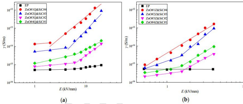
Figure 2. \gamma -E characteristic curves of composite materials with different proportions of inorganic fillers: (a) nano-ZnO/SiC/EP nanocomposites; (b) micro-ZnO/SiC/EP micro/nanocomposites [33].
