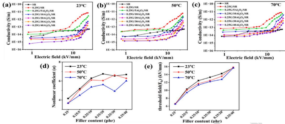
Figure 3. DC conductivity at (a) 23 °C, (b) 50 °C, (c) 70 °C, and (d) The nonlinear coefficient \alpha and (e) the threshold field strength E_b of the G/ \text{Al}_2\text{O}_3 /SR composites[39].
