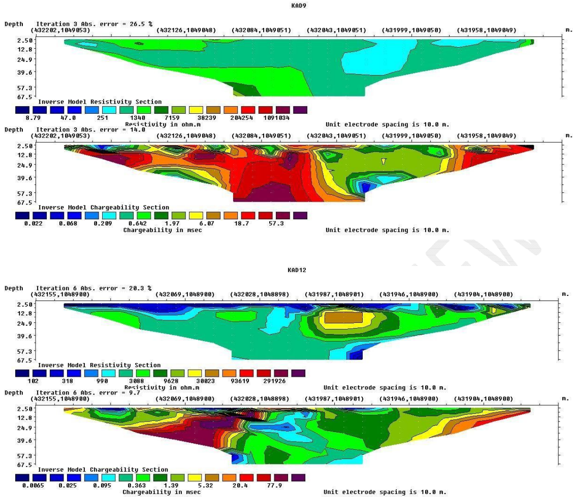
Figure 6: ERT/IP inversion model for the [redacted]
