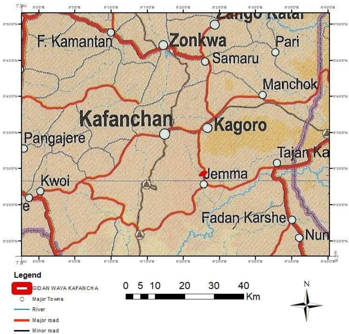
Figure 1: Location map of the study area with towns and villages modified after (NGSA, 2006)
