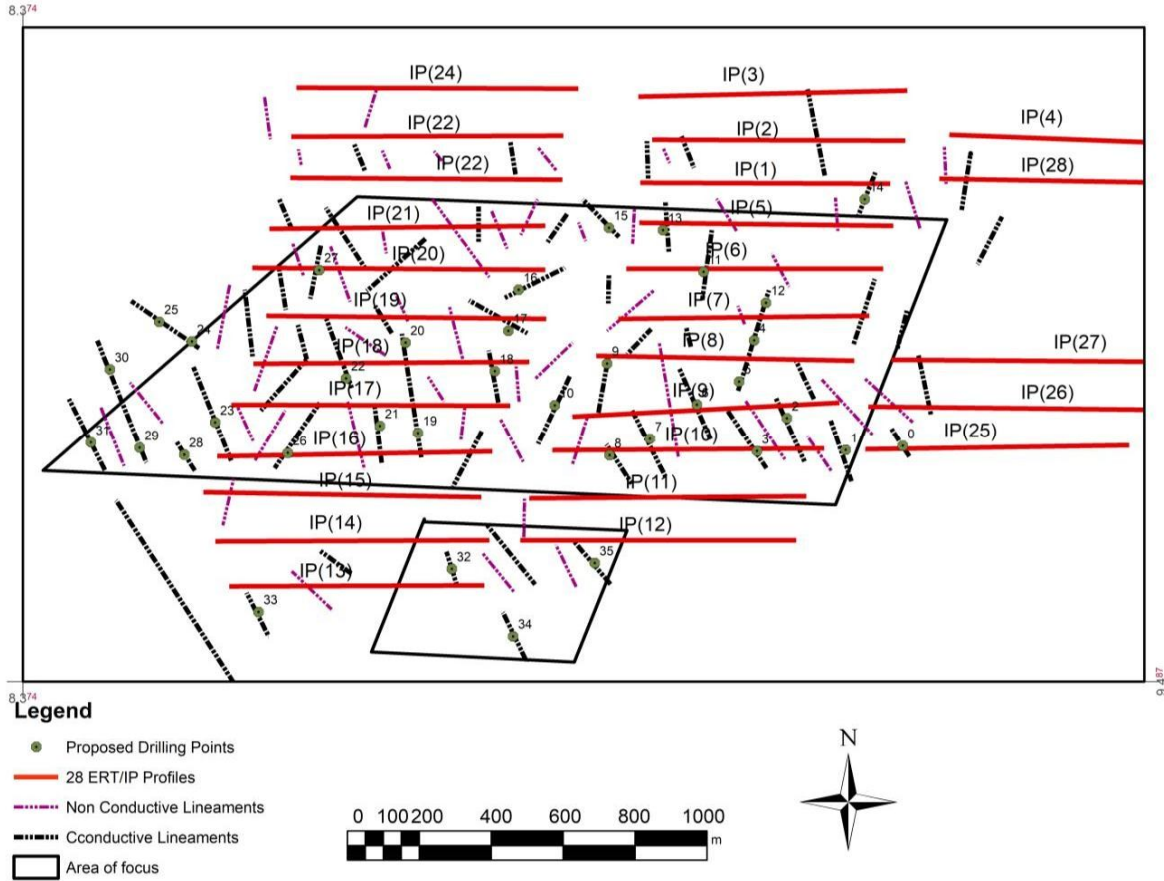
Figure 7: Mineral Prospective Interpreted Map
