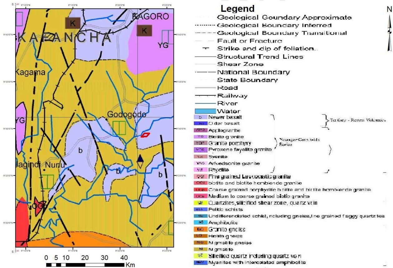
Figure 2: Geological map and Mineral Resources Map with the Study Area in Red Rectangle (Modified after NGSA, 2023)
