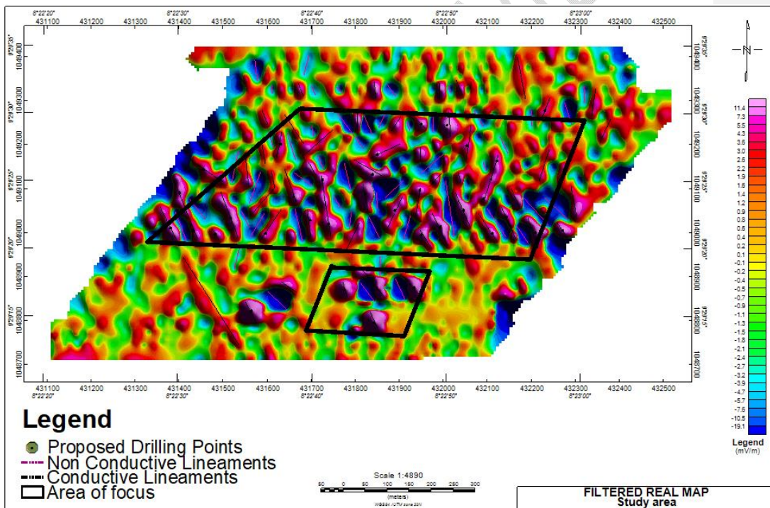
Figure 3: Filtered real Map
