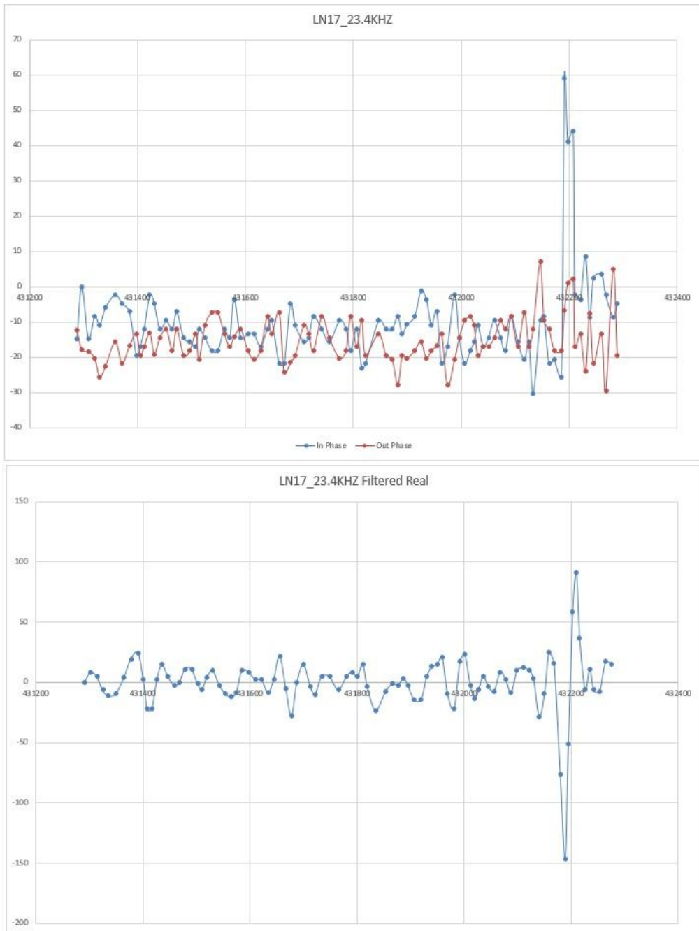
Figure 5: In phase, quadrature and filtered real of Ln17_23.4khz
