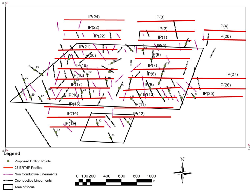
Figure 7: Mineral Prospective Interpreted Map
