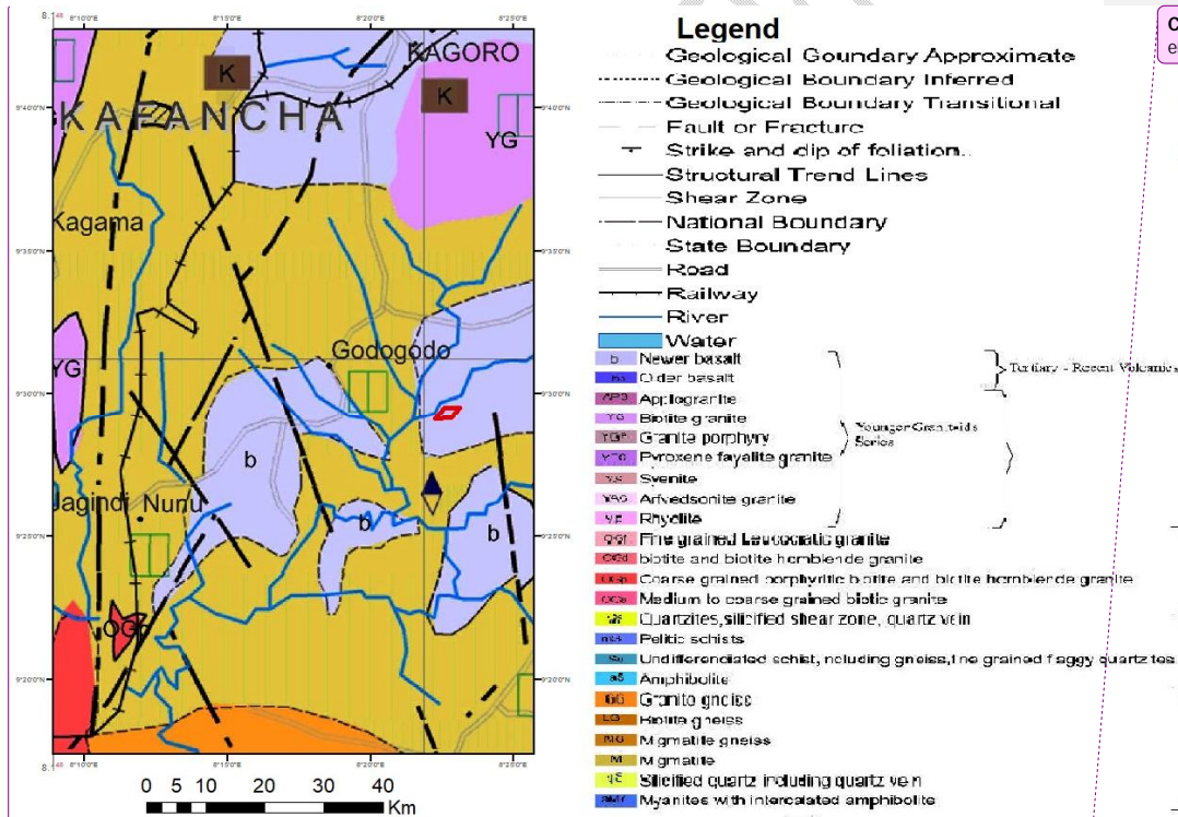
Figure 2: Geological map and Mineral Resources Map with the Study Area in Red Rectangle (Modified after NGS, 2023)
