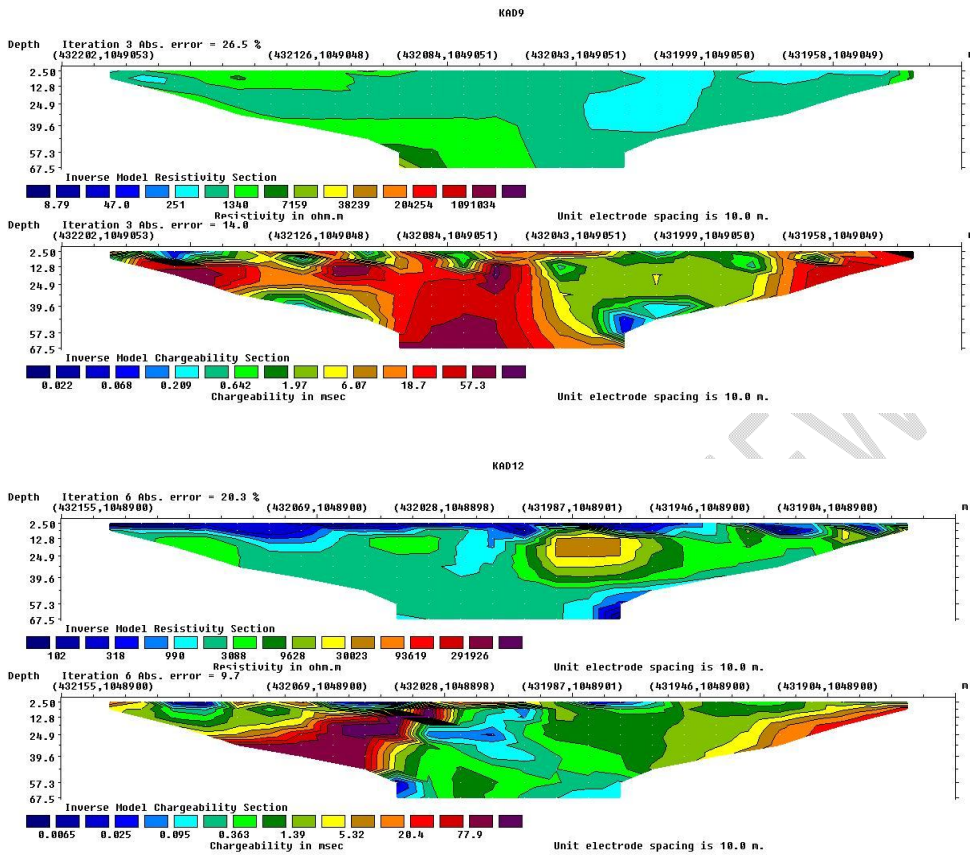
Figure 6: ERT/IP inversion model for the selected profiles
