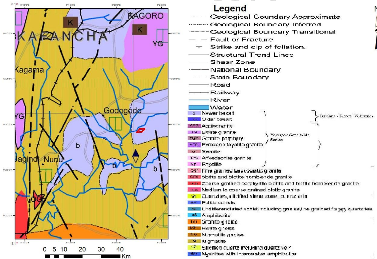
Figure 2: Geological map and Mineral Resources Map with the Study Area in Red Rectangle (Modified after NGSA, 2023)
