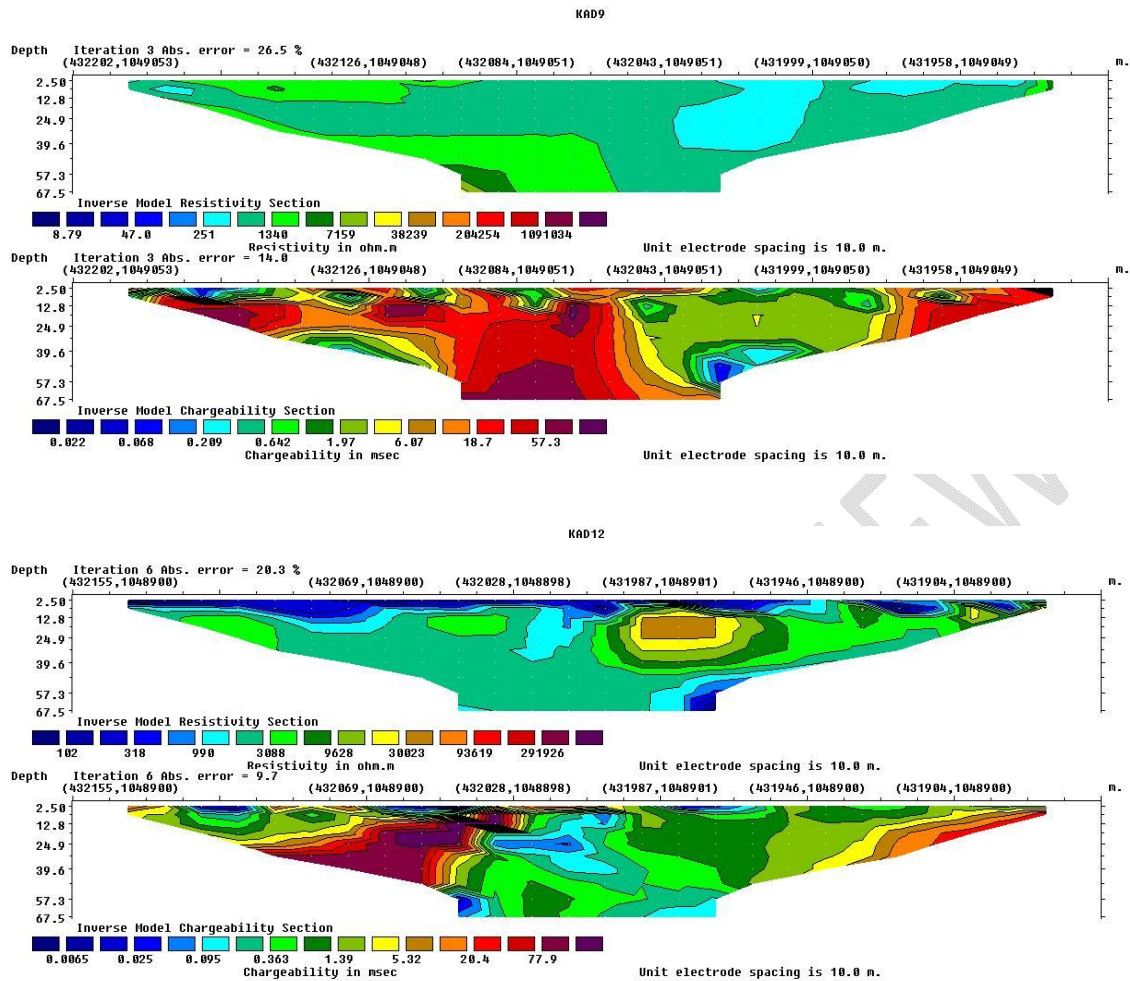
Figure 6: ERT/IP inversion model for the selected profiles
