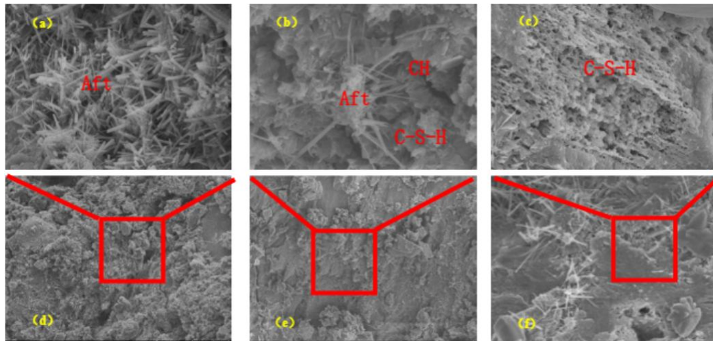
Fig.7 Surface micromorphological changes
