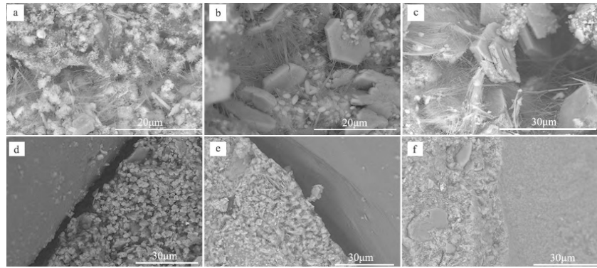
Fig.6 Morphology of recycled mortar
