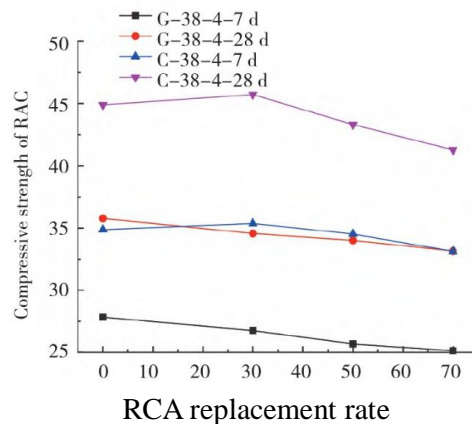
Fig.2 Compressive strength of recycled concrete with different gradation forms Zhang et al [32] conducted strength tests on recycled concrete with different
