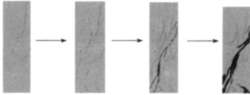
Fig.1 Typical failure process and appearance of recycled concrete prisms
