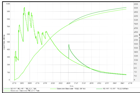
Figure 5. Rate and Total Oil Production in Field “RK” Scenario I
