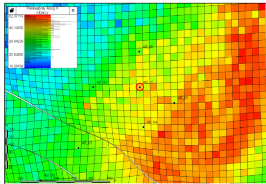
Figure 4. Permeability Distribution Map Around Well AB_05
