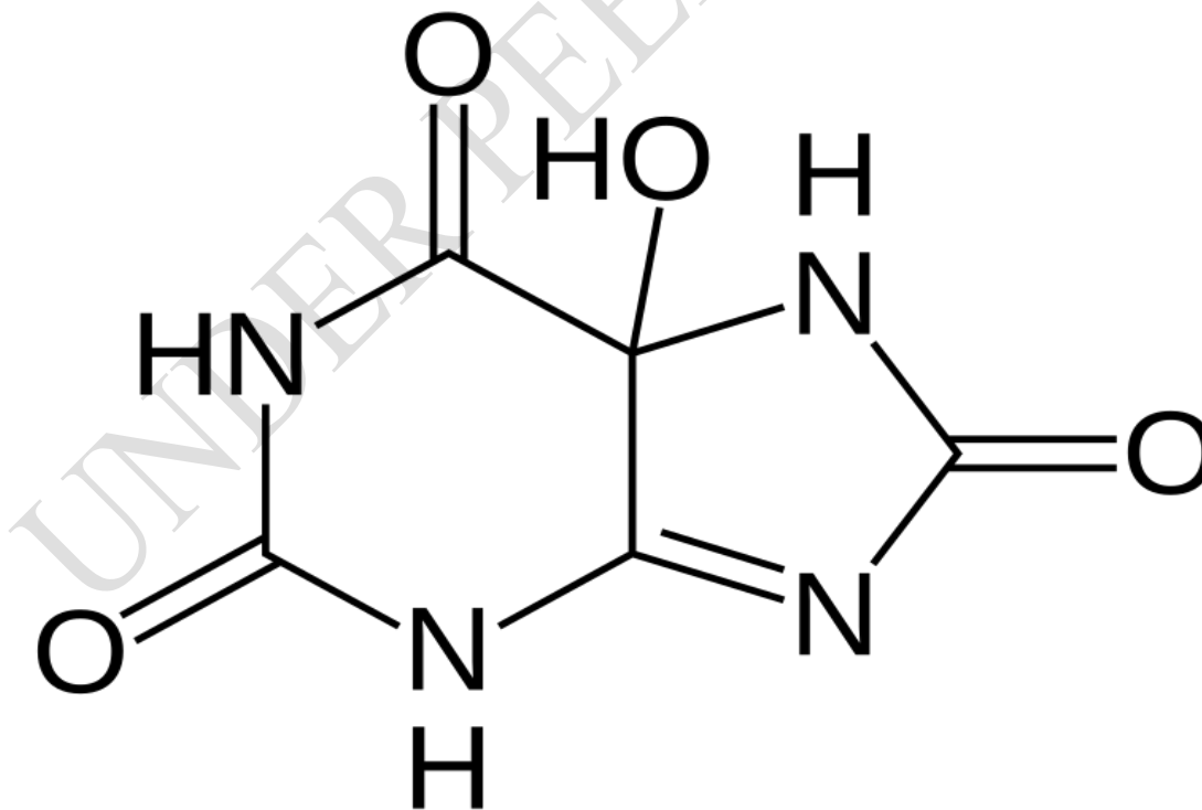
Figure 1: 5-Hydroxyisourate chemical formula [13].
