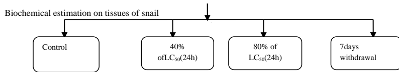
Chart 1 : Study protocol
