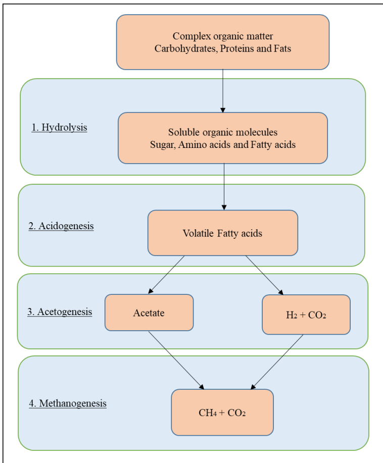
Fig. 7 Biogas production technology.
