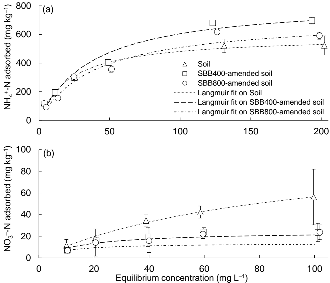
Figure 3. (a) Adsorption isotherms for \text{NH}_4^+\text{-N} on soil only, SBB400-amended soil, and SBB800-amended soil. (b) Adsorption isotherms for \text{NO}_3^-\text{-N} on soil only, SBB400-amended soil, and SBB800-amended soil.
