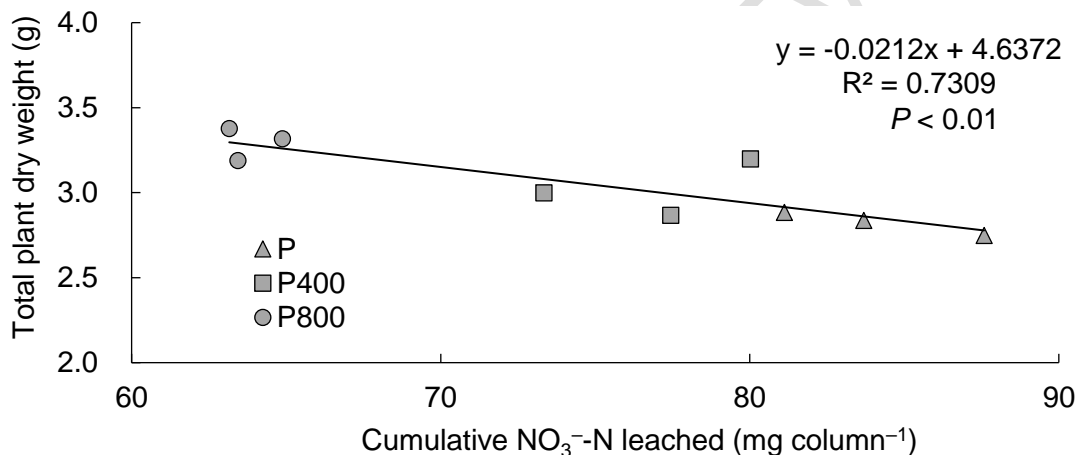
Figure 5. Relationships between cumulative \text{NO}_3^- -N leached and total plant dry weight grown on soil only, SBB400-amended soil, and SBB800-amended soil. SBB400 and SBB800 are bagasse biochar pyrolyzed at 400°C and 800°C, respectively.
