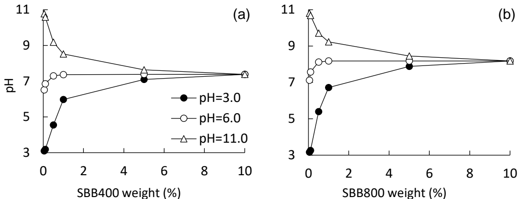
Figure 1. (a) Mass titration curves for SBB400. (b) Mass titration curves for SBB800. SBB400 and SBB800 are bagasse biochar pyrolyzed at 400°C and 800°C, respectively.
