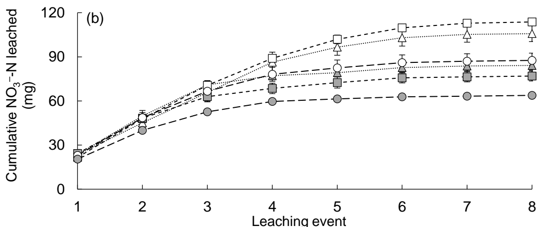
Figure 4. (a) Cumulative amounts of \text{NH}_4^+\text{-N} leached from the columns with 8 leaching events. (b) Cumulative amounts of \text{NO}_3^-\text{-N} leached from the columns with 8 leaching events
