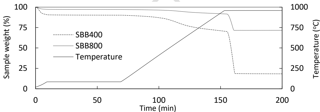
Figure 2. Thermal gravimetric curves for SBB400 and SBB800.
