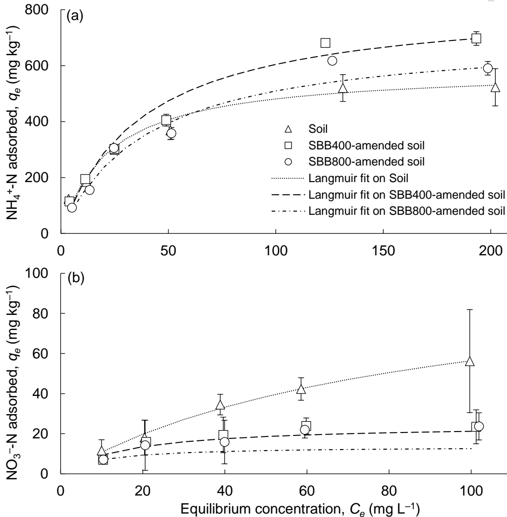
Figure 1. Adsorption isotherms for (a) \text{NH}_4^+\text{-N} and (b) \text{NO}_3^-\text{-N} on soil only, SBB400-amended soil, and SBB800-amended soil
