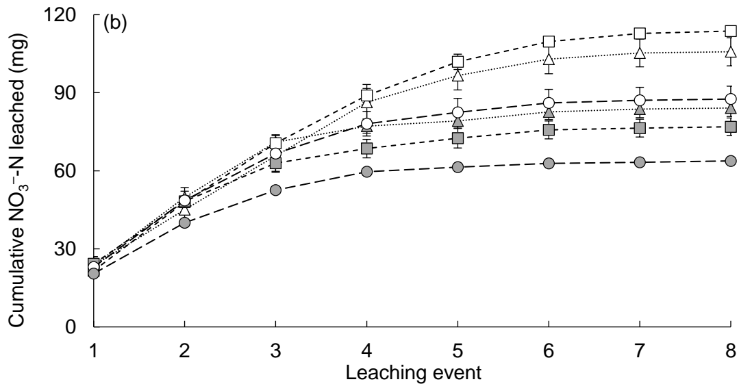
Fig. 2. Cumulative amounts of (a) NH 4 + -N and (b) NO 3 - -N leached from the columns with 8 leaching events
