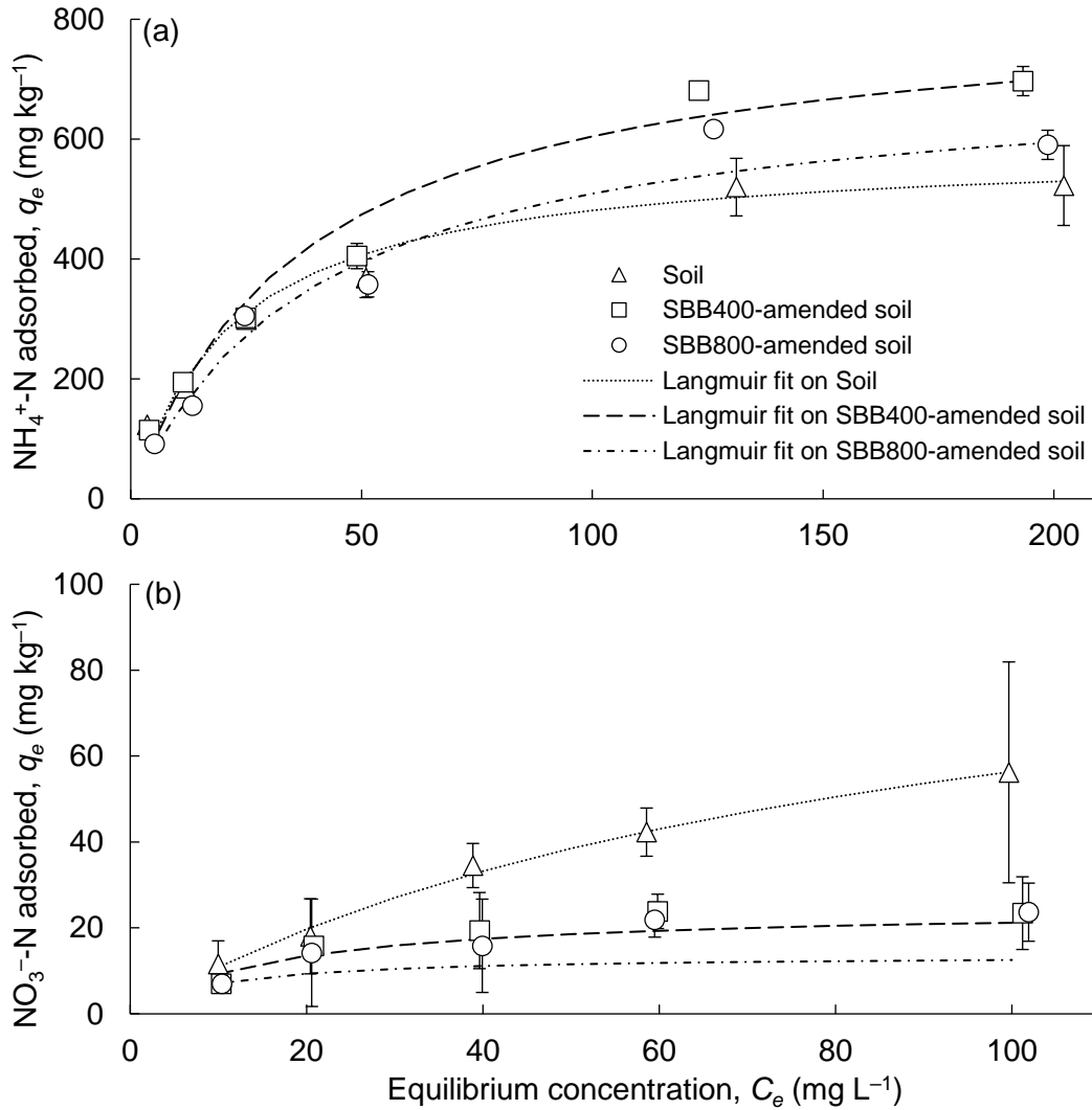
Fig. 1. Adsorption isotherms for (a) \text{NH}_4^+\text{-N} and (b) \text{NO}_3^-\text{-N} on soil only, SBB400-amended soil, and SBB800-amended soil
