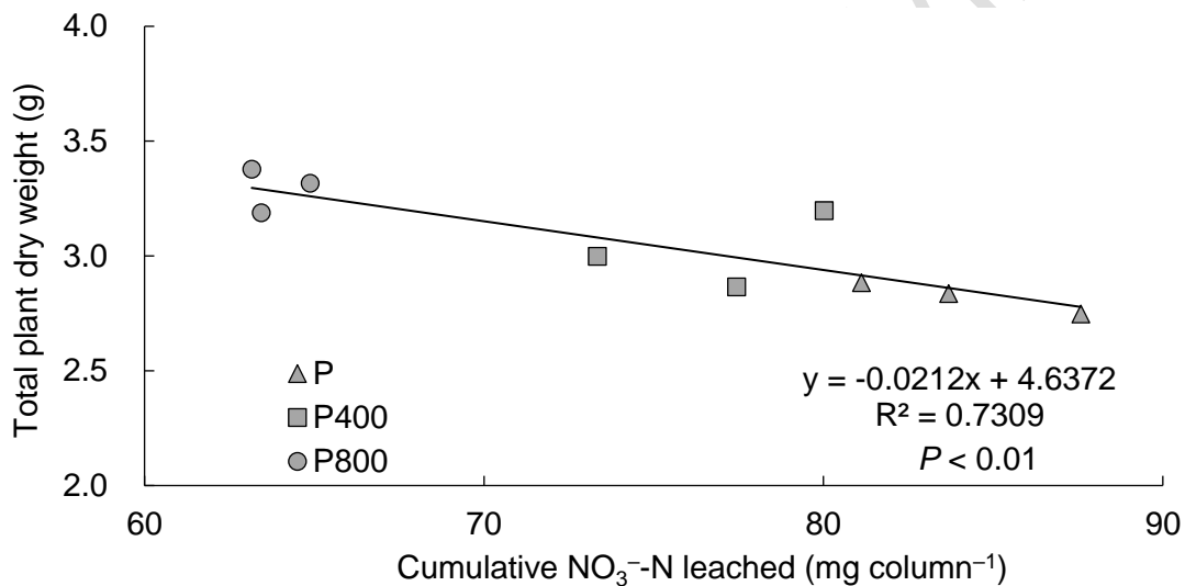
Fig. 3. Relationships between cumulative \text{NO}_3^- -N leached and total plant dry weight grown on soil only, SBB400-amended soil, and SBB800-amended soil
