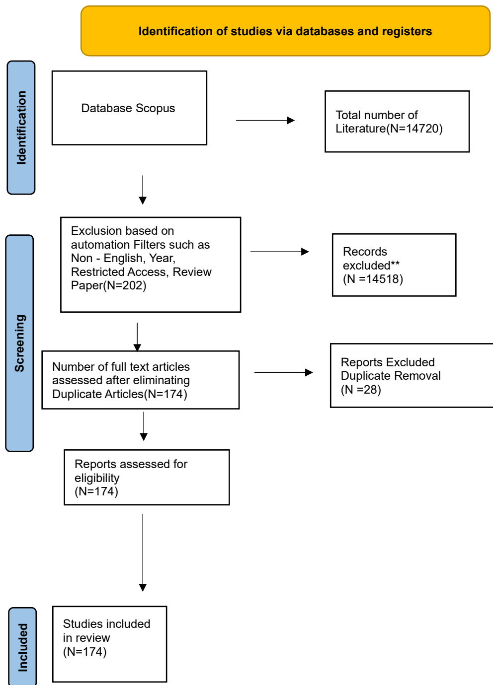
Fig 1: PRISMA FLOWCHART
