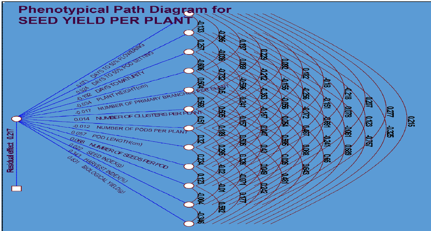
Fig 1 Phenotypic path diagram for seed yield per plant
