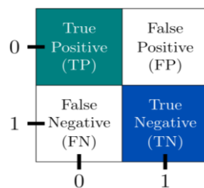
Figure 12: Confusion Matrix General Form
