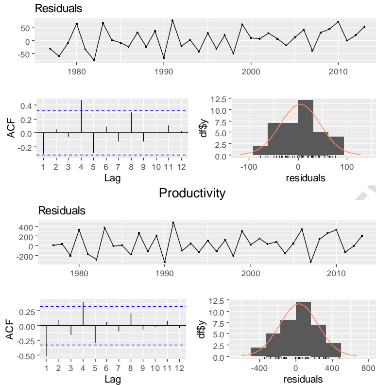
Fig. 7: Residual plots, ACF plots, and distribution of standardized residuals of AR (1) - GARCH (1,1) models for Aman rice area, production, and productivity in Jalpaiguri
