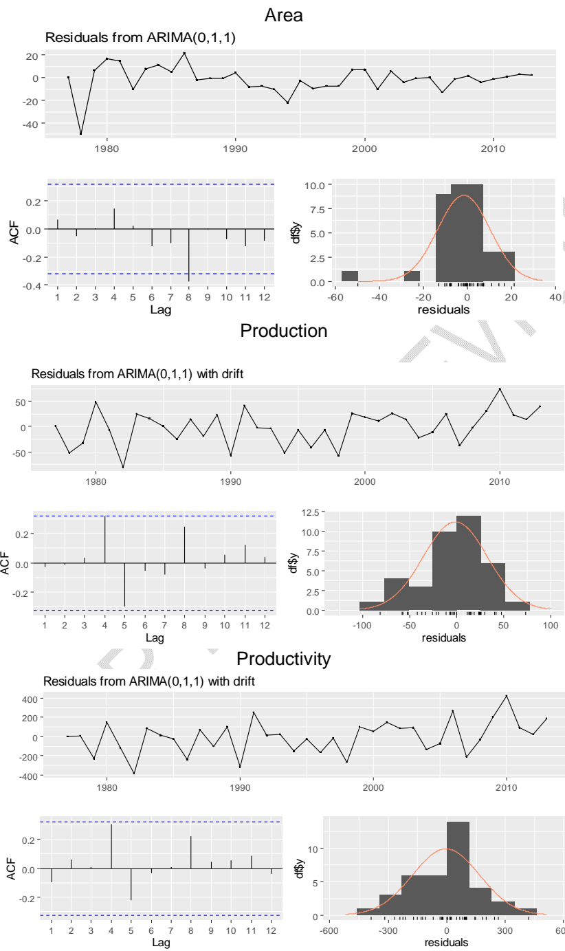
Fig. 3: Residual plots, ACF plots, and distribution of ARIMA (0,1,1), ARIMA (0,1,1), and ARIMA (0,1,1) for Aman rice area, production, and productivity in Jalpaiguri
