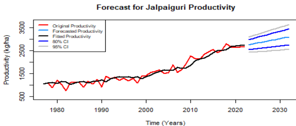
Fig. 7: Forecast plot of AR (1) - GARCH (1,1) of Aman rice Area, AR (1) - GARCH (1,1) of Production, ARIMA (0,1,1) of Productivity for Jalpaiguri
