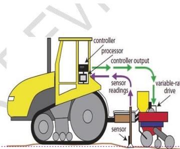
Figure 10: VRT hardware in tractor
