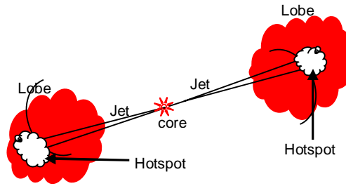
Fig. 2. The structure of a typical extragalactic radio source. Source: The authors
