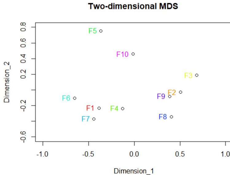
Figure 7: Two-dimensional MDS plot for the practical dataset
