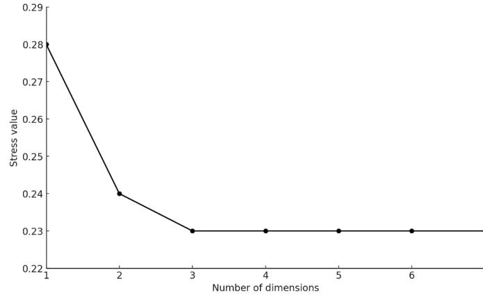
Figure 1: Scree-plot
