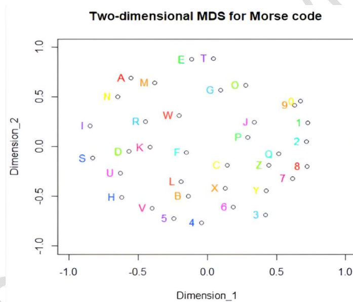
Figure 4: Result of applying MDS to the proximities of Morse code data
