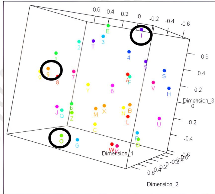
Figure 5: Three-dimensional MDS plot for Morse code data
