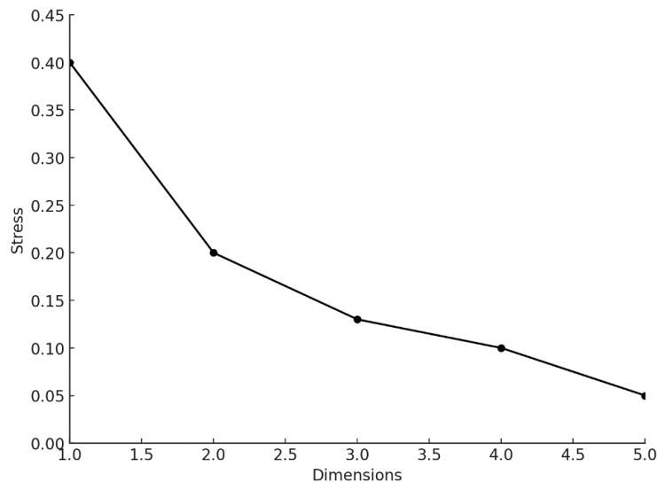
Figure 6: Scree-plot obtained for the practical dataset
