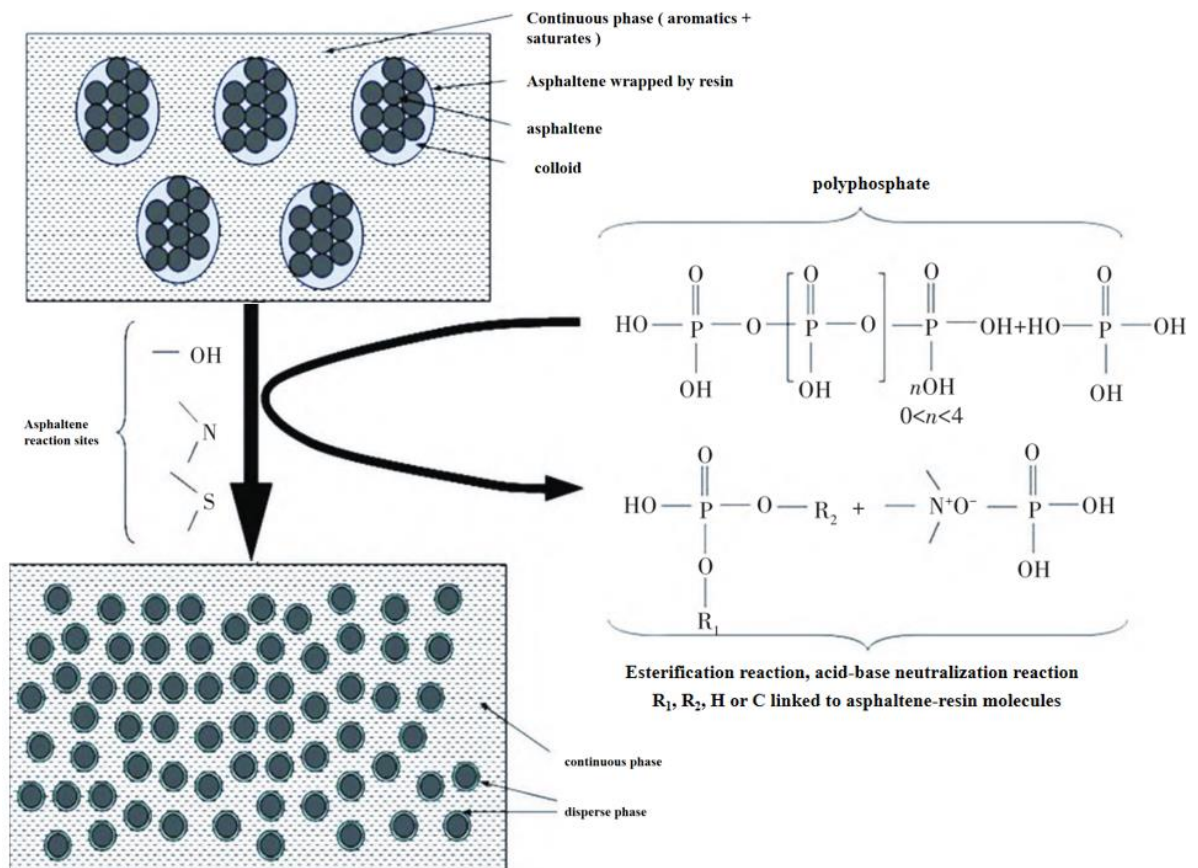
Fig.1 Effect of PPA on asphalt composition [37]
