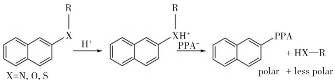
Fig.2 Acidolysis and nucleophilic substitution of alkylarenes
