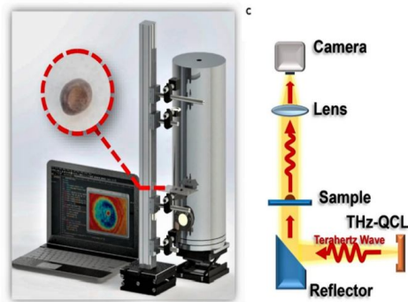
Fig 4: THz QCL video imaging system
