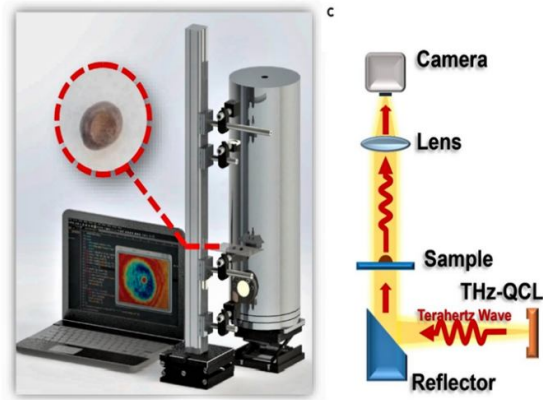
Fig 4: THz QCL video imaging system
