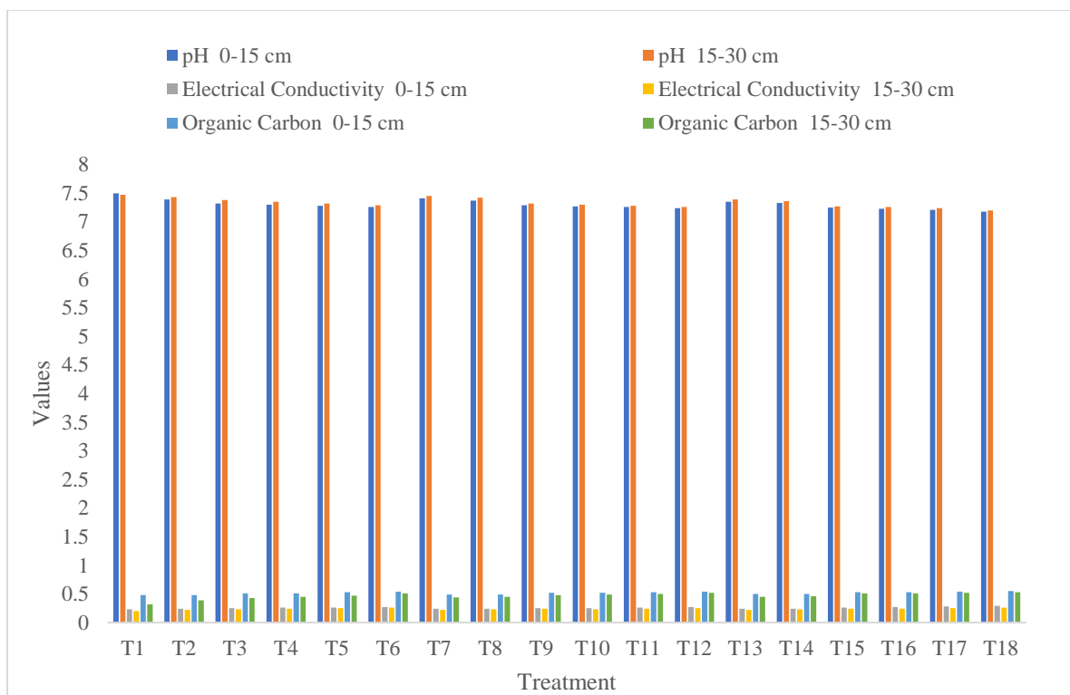
Fig-3. Effect of NPK, Rhizobium and FYM on Physico-Chemical Properties of Soil for Cluster Bean ( Cyamopsis tetragonoloba L.) Cv. Radha SPL on pH, electrical conductivity, organic compound of soil after crop harvest.
