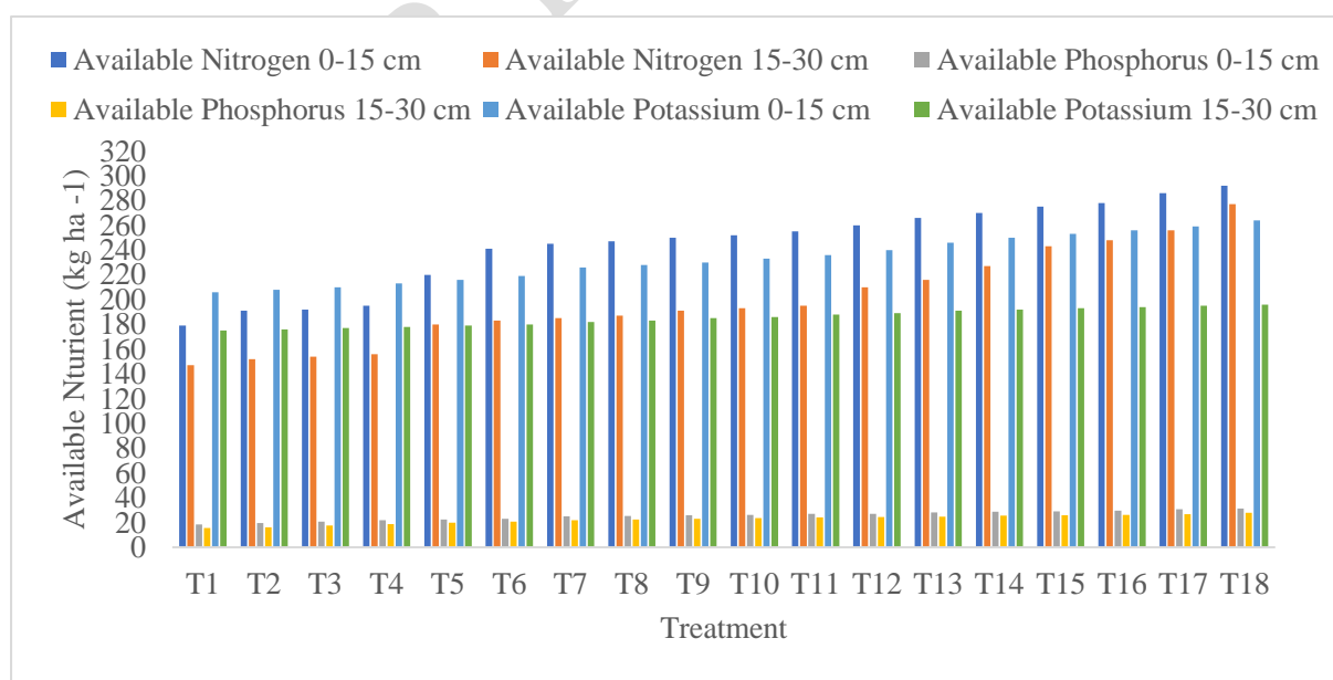
Fig-4. Effect of NPK, Rhizobium and FYM on Physico-Chemical Properties of Soil for Cluster Bean ( Cyamopsis tetragonoloba L.) Cv. Radha SPL on Nitrogen, Phosphorous
