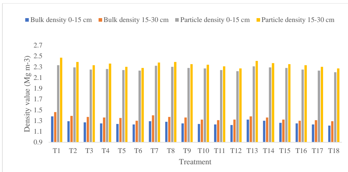
Fig-1. Effect of NPK, Rhizobium and FYM on Physico-Chemical Properties of Soil for Cluster Bean ( Cyamopsis tetragonoloba L.) Cv. Radha SPL on bulk density, particle density of soil after crop harvest
