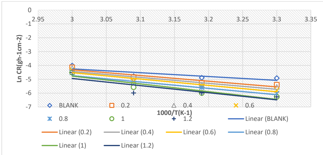
Fig. 9: Relationship between \ln CR and 1/T for mild steel in 1 M HCl solution in different concentration of TG dye
