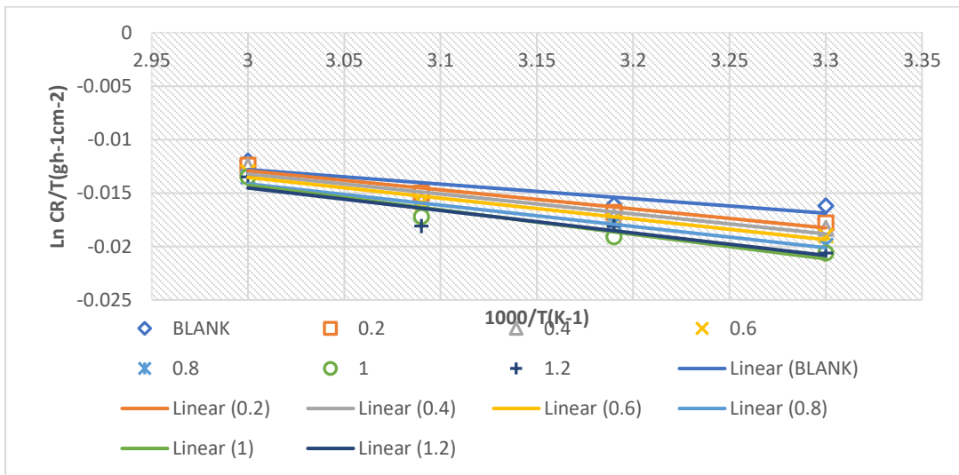
Fig.10: Relationship between \ln CR/T and 1/T for mild steel in 1 M HCl solution in different concentration of TG dye
