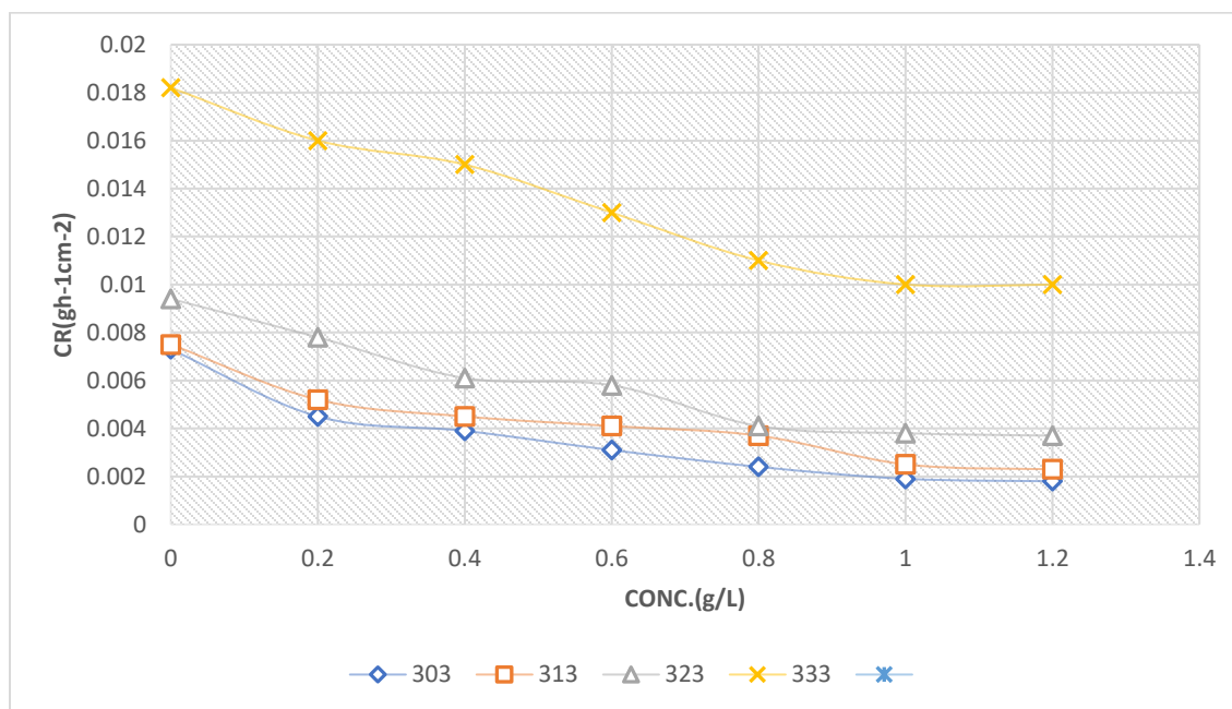
Fig.3: Effect of TG dye on corrosion rate
