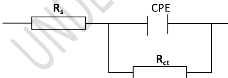
Fig. 8: The equivalent circuit diagram
