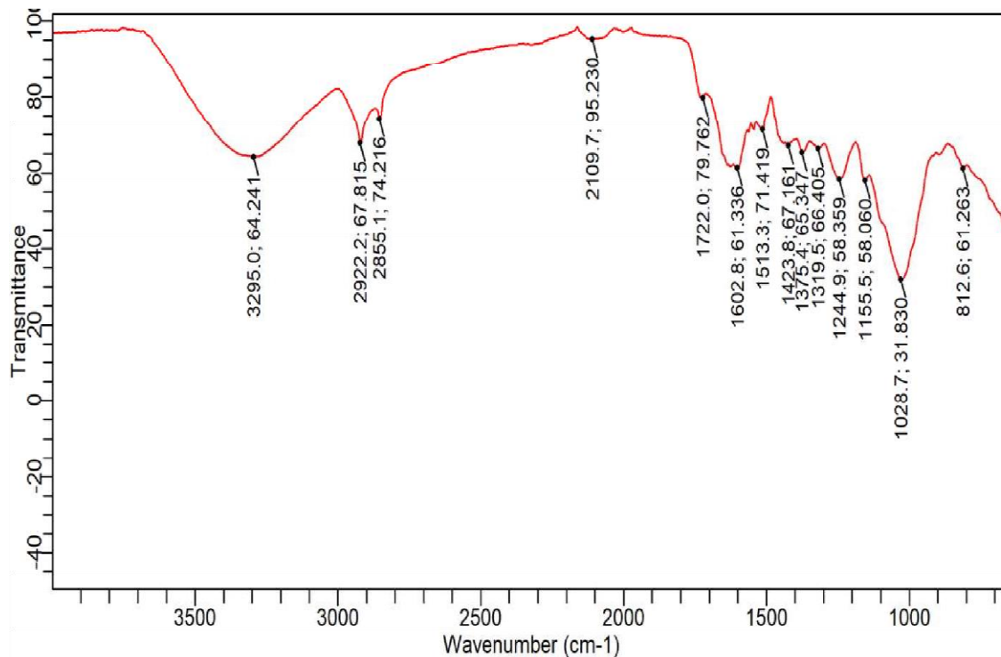
Fig. 2: FTIR spectrum of TG dye
