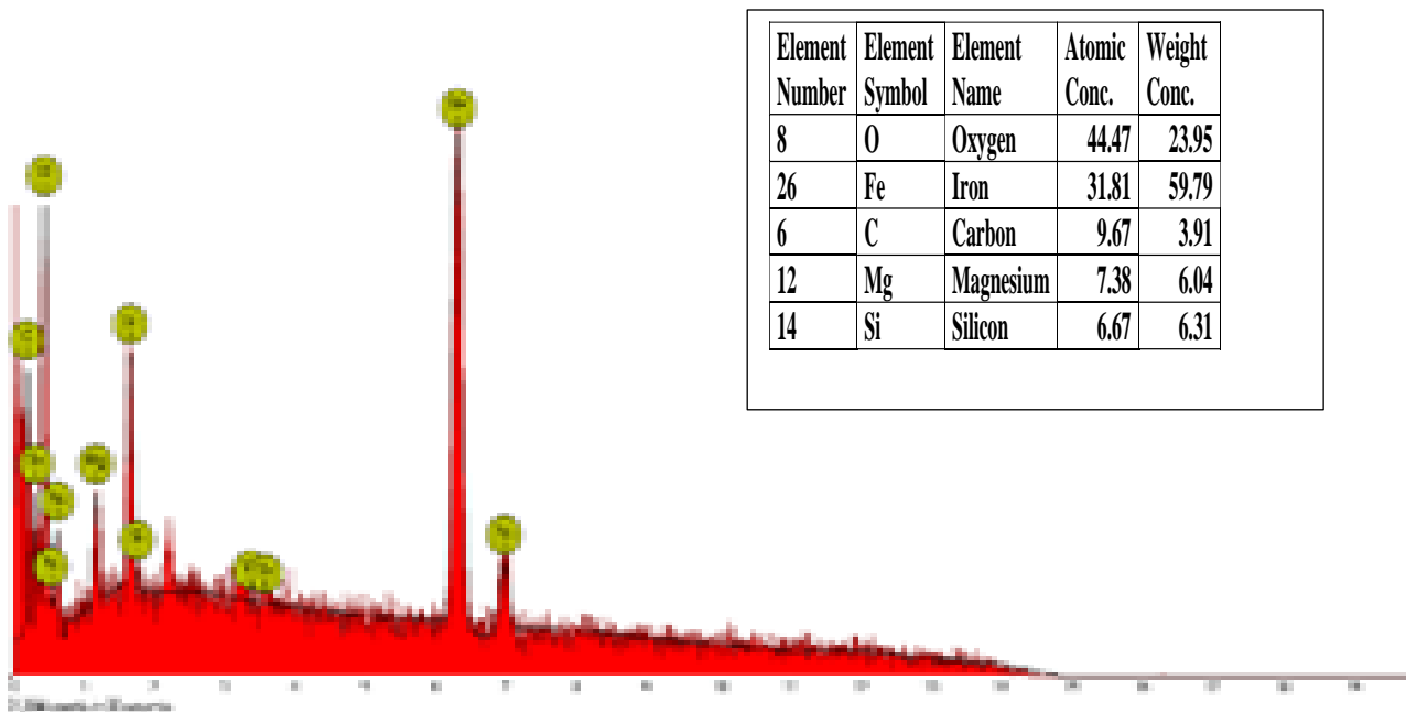
Fig14(c): SEM image and EDX analysis of Mild steel after immersion into TG Dye inhibitor solution
