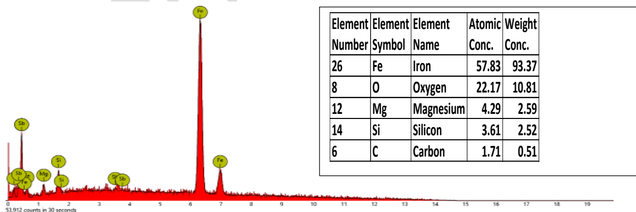
Fig 14(a): SEM image and EDX analysis of mild steel
