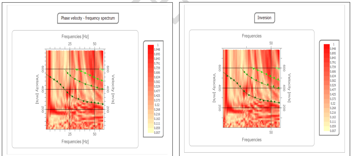
Figure 3b: Dispersion curve illustrating the variation of shear wave velocity with frequency
