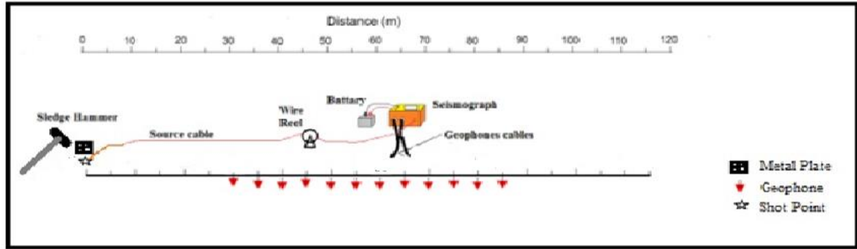
Figure 2: Equipment setup for MASW
