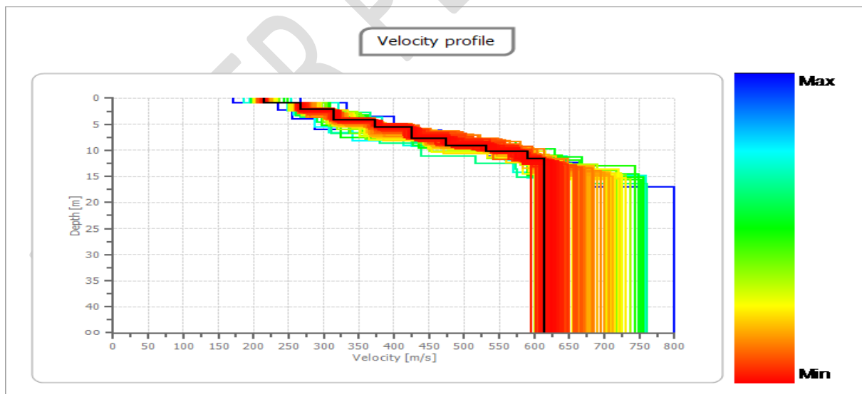
Figure 4b: Velocity model from seismic refraction survey in Amassoma
