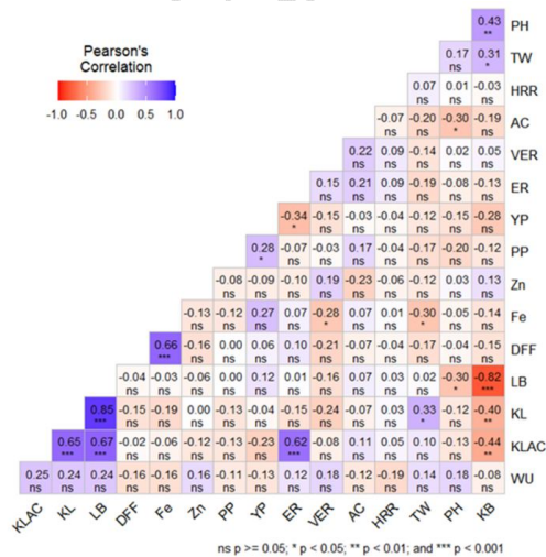
Fig 3 Pearson's correlation plot for yield, yield component and quality traits
