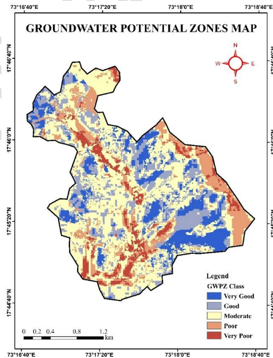
Fig. 10: Groundwater potential zone map of Wakawali watershed
