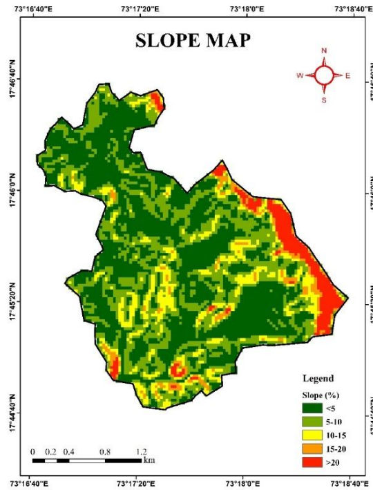
Fig. 3: Spatial distribution map of slope
