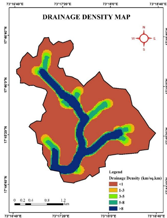
Fig. 4: Spatial distribution map of drainage density
