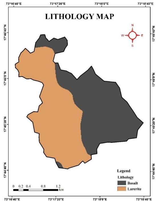
Fig. 5: Spatial distribution map of lithology
