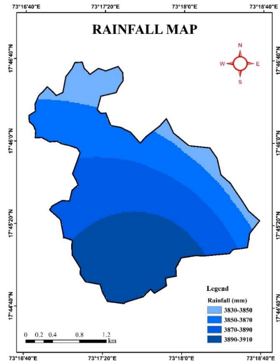
Fig. 8: Spatial distribution map of rainfall
