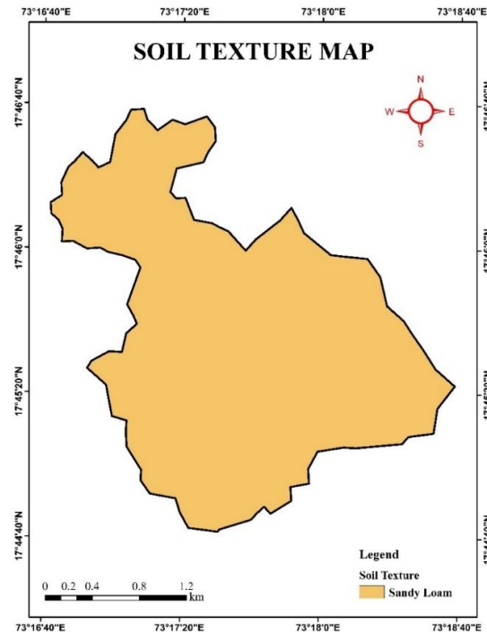
Fig. 7: Spatial distribution map of soil texture
