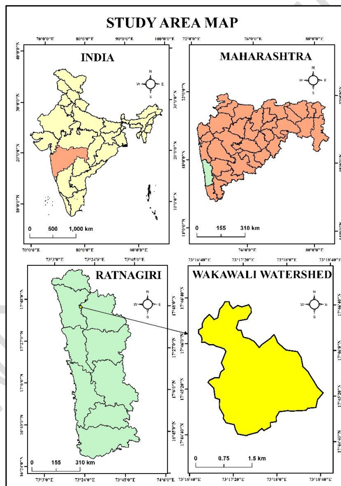
Fig. 1: Location map of Wakawali watershed
