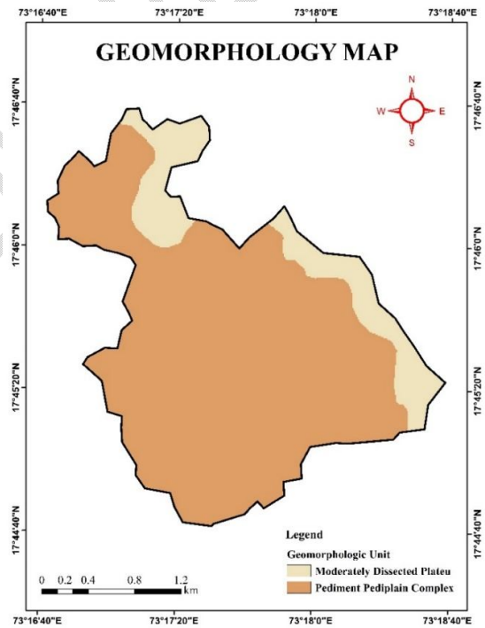
Fig. 6: Spatial distribution map of geomorphology
