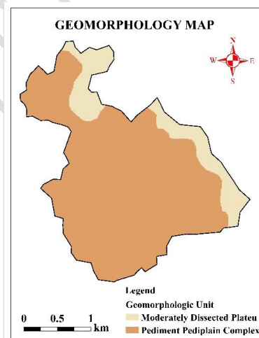
Fig. 6: Spatial distribution map of geomorphology
