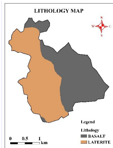
Fig. 5: Spatial distribution map of lithology
