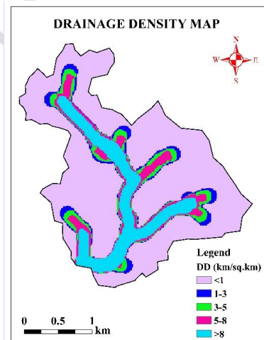
Fig. 4: Spatial distribution map of drainage density
