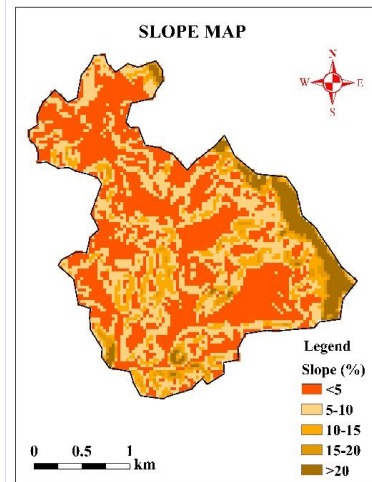
Fig. 3: Spatial distribution map of slope
