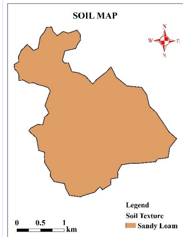
Fig. 7: Spatial distribution map of soil texture
