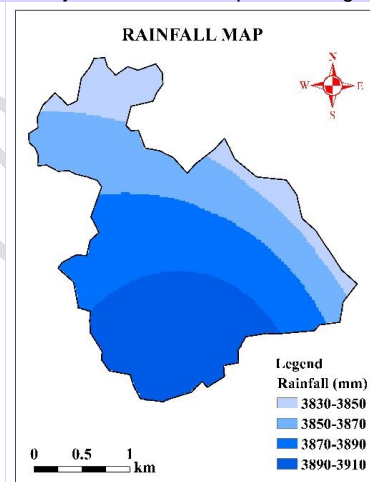
Fig. 8: Spatial distribution map of rainfall
