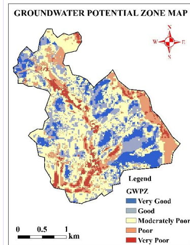
Fig. 10: Groundwater potential zone map of Wakawali watershed
