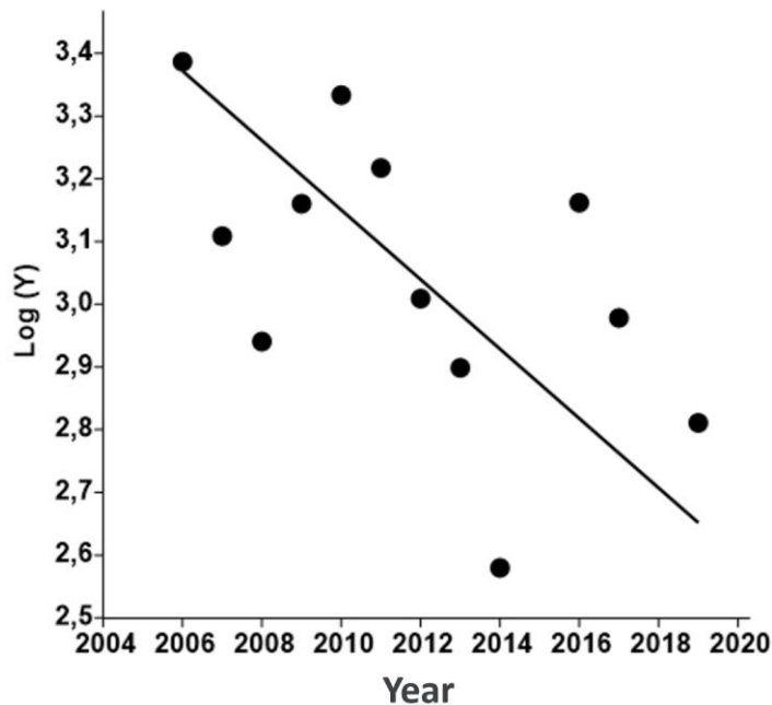
Figure 33: Trend in the waterbuck population from 2006 to 2019; Ln (Y) is the estimated waterbuck population size
