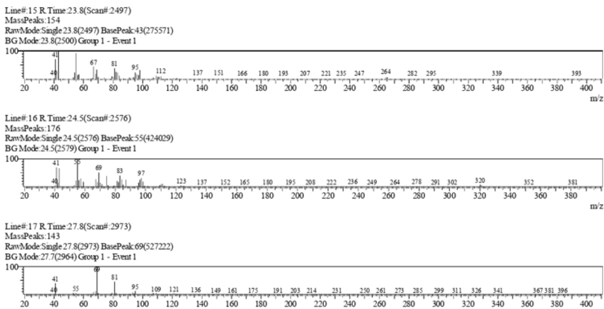
Figure 3: Mass spectra of the 17 identified compounds indicated by the GC peaks
