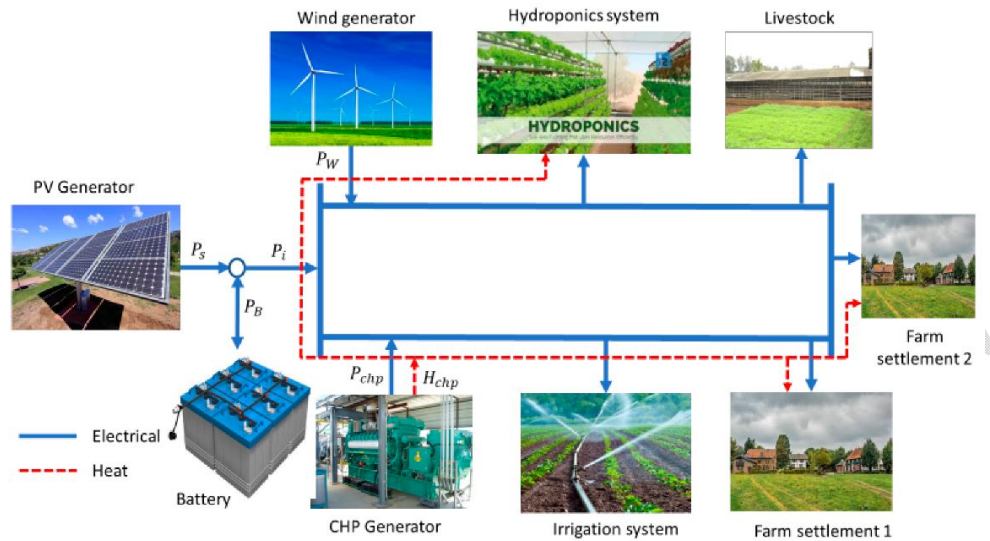
Fig. 13. Diagram of a prototype set up of hybrid PV solar/ wind and battery system
