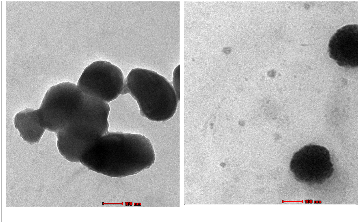
Plate 2a. TEM images of Spirulina platensis mediated TiO 2 NPs
