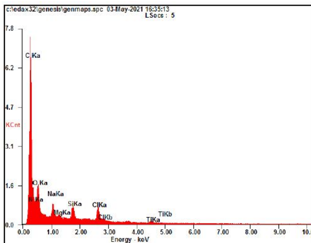
Plate 2b. TEM with EDAX element of Spirulina platensis mediated TiO 2 NPs
