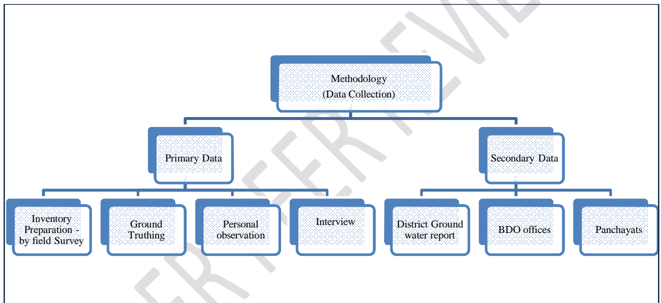
Fig. 2 Methodology
