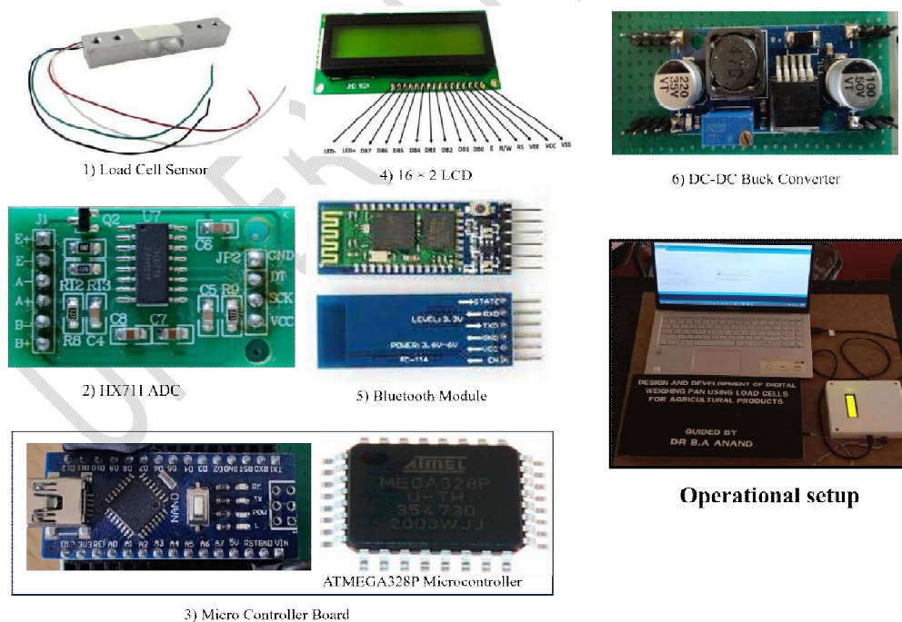
Figure 1: Components and operational setup of Microcontroller-Based Weight Measurement System for liquid Agriculture produce
