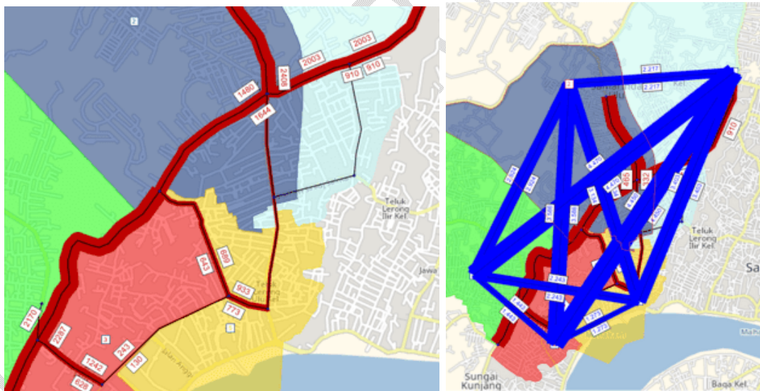
Figure 4. Existing Traffic Performance (Source: PTV Vissum analysis results, 2023)
