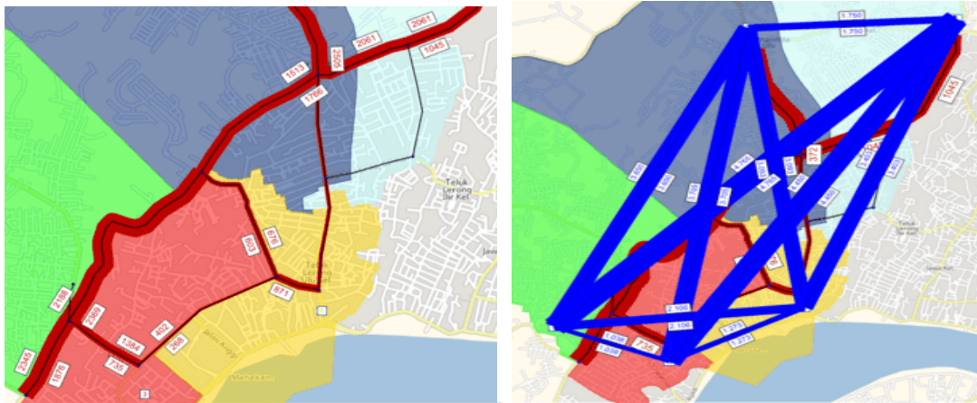
Figure 9. Traffic Performance for the Operational Period (Do Nothing) in 2034 (Source: PTV Vissum analysis results, 2023)
