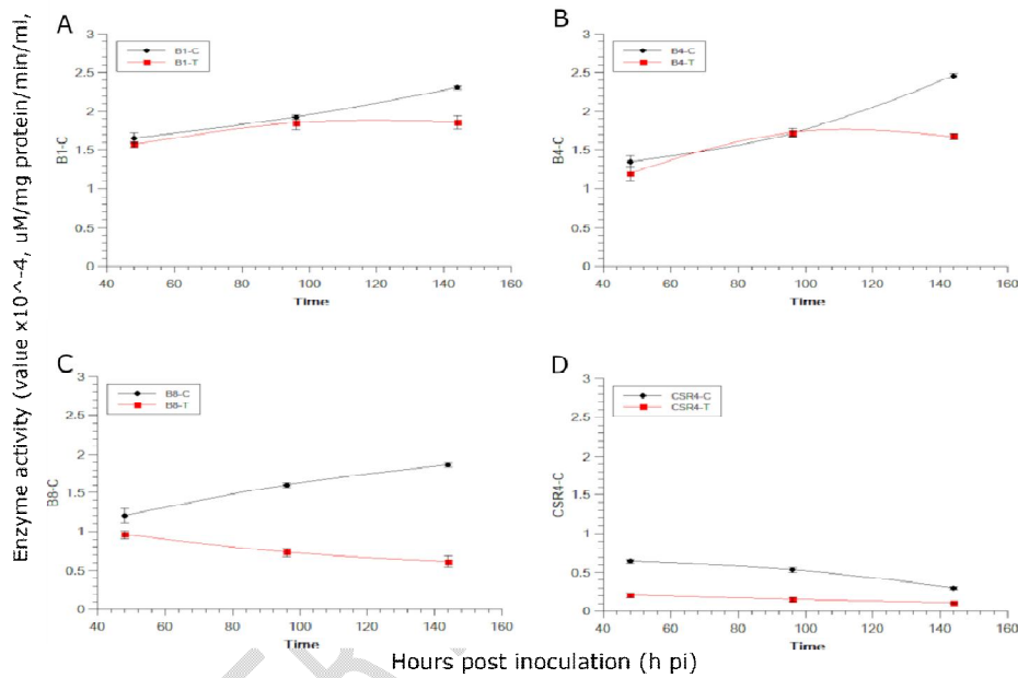
Fig. 3: Trehalase activity (µM/mg protein/min/ml) in selected thermotolerant bivoltine silkworm breeds as influenced by B. bassiana inoculation at different time intervals
