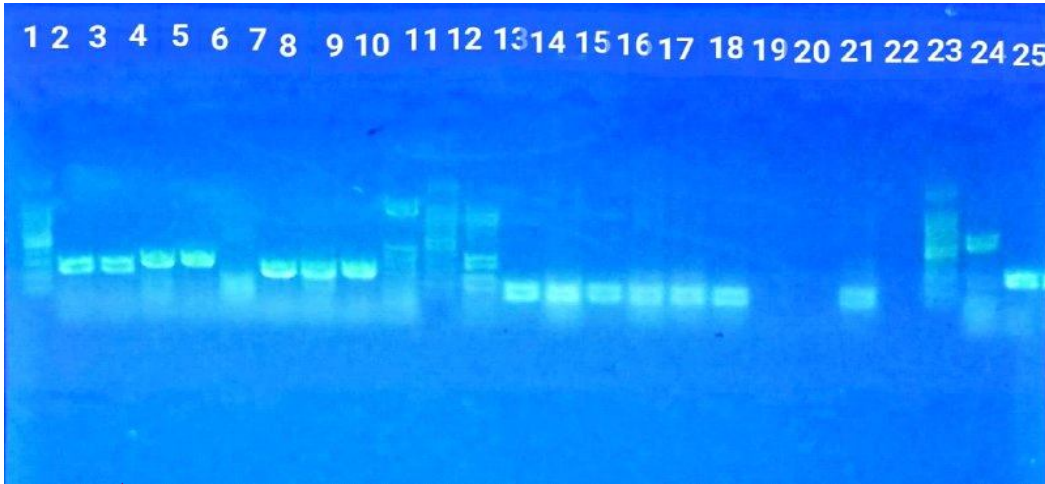
Fig (1): Agarose gel electrophoresis of multiplex PCR product: 1, 12, 23=100 bp ladder, 2 positive control of Staph aureus , 3,4,5,7,8,9,25 are positive Staph aureus 13, 14, 15, 16, 17, 18, 21 positive E.coli .
