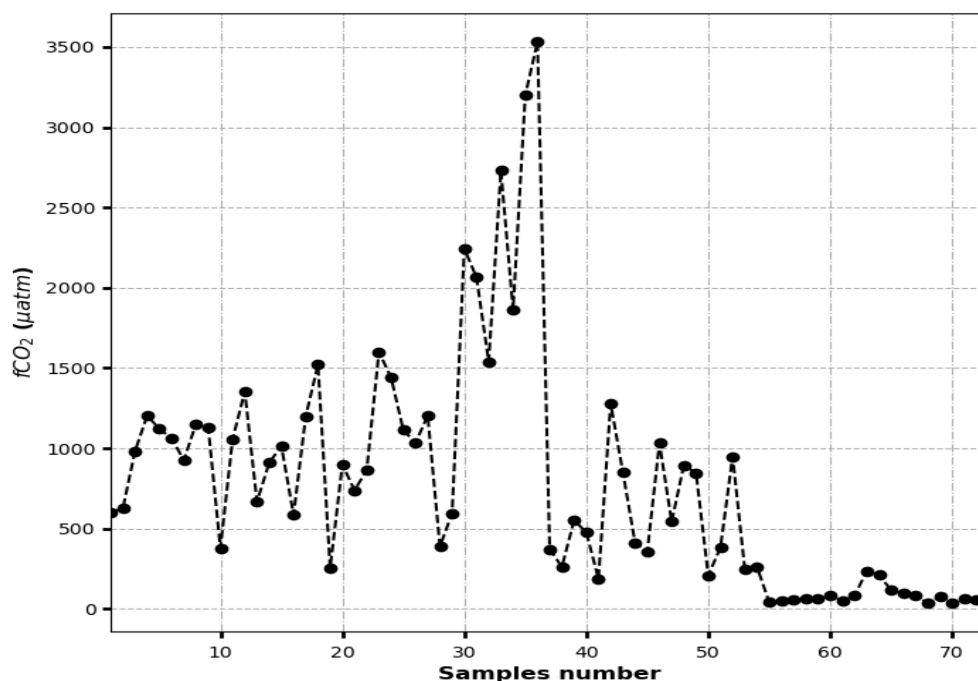
Fig. 4. Calculated fugacity of CO 2 (fCO 2 ) in Vridi channel
