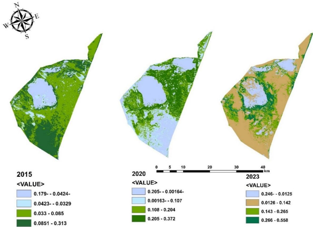
Figure3. NDVI classification in the study area.
