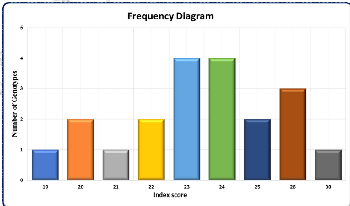
Figure 2:FrequencydiagramwithIndexscoreandnumberofgenotypes:
