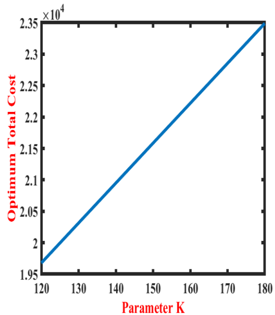
Figure 11 Changes of Optimum Total Cost with Parameter K
