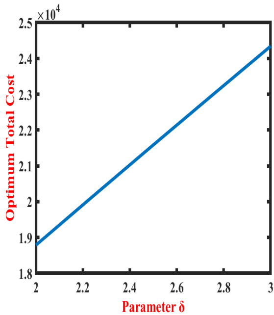
Figure 10 Changes of Optimum Total Cost with Parameter \delta
