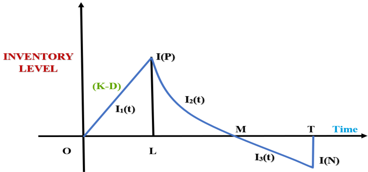
Figure 1: Production Inventory Model with Shortage Allowed
