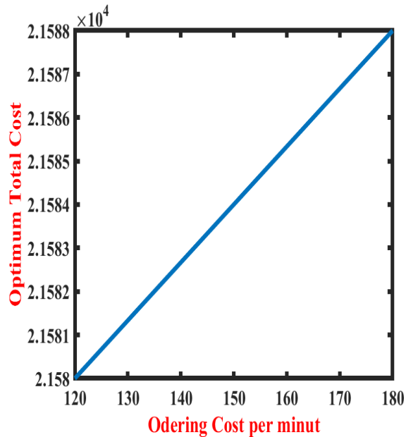
Figure 2 Changes of Optimum Total Cost with Odering Cost.
